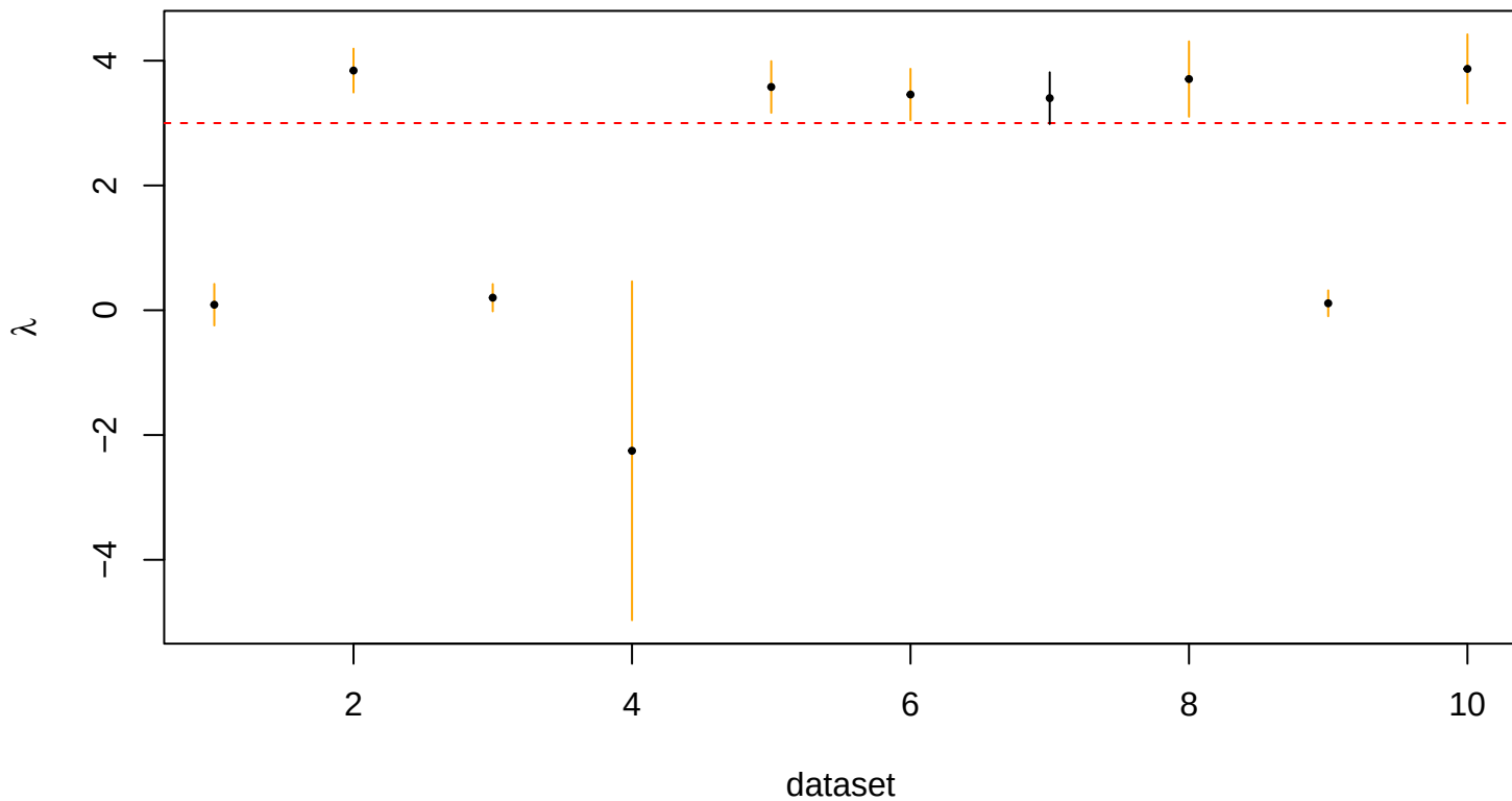
95% CI for lambda – method 8, mrts_k = 0
