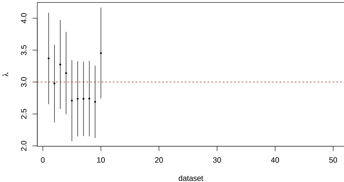
95% CI for lambda – method 2, mrts_k = 10
