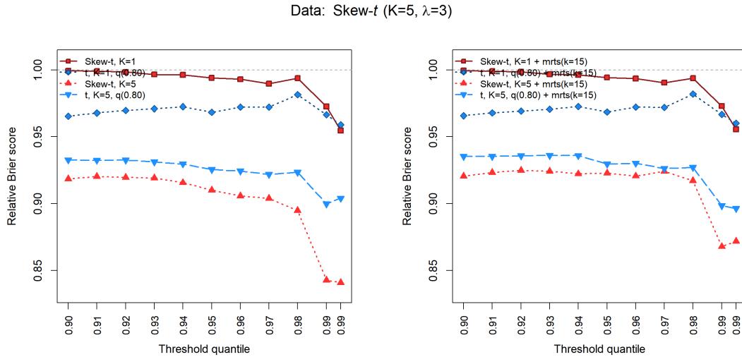
(b) Setting 5 (data-generating process: skew- t with K = 5 knots, \lambda = 3 ). Relative Brier scores of methods 2–5 versus the Gaussian baseline; left panel is the no-MRTS baseline, right panel adds an MRTS basis of rank K_{\text{MRTS}} = 15 . The matching five-knot skew- t method (method 4) is decisively the best across all quantiles, with relative Brier scores between roughly 0.84 and 0.92. All four methods improve on the Gaussian baseline, in contrast with setting 4 where the over-specified method 5 was worse than Gaussian. The right panel mirrors the left panel closely, indicating that the MRTS basis adds little beyond what the spatial skew- t structure already captures.
