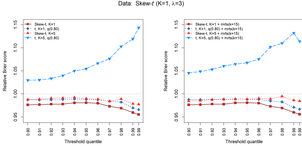
(a) Setting 4 (data-generating process: skew- t with K = 1 knot, \lambda = 3 ). Relative Brier scores of methods 2–5 versus the Gaussian baseline at threshold quantiles 0.90 \leq q \leq 0.995 , with K_{\text{MRTS}} = 15 . The left panel shows the no-MRTS baseline and the right panel shows the same methods with the MRTS basis added. The matching method (skew- t with K = 1 , method 2) is best at every quantile, the over-specified five-knot threshold- t method (method 5) is worse than Gaussian, and the right panel is nearly indistinguishable from the left.
