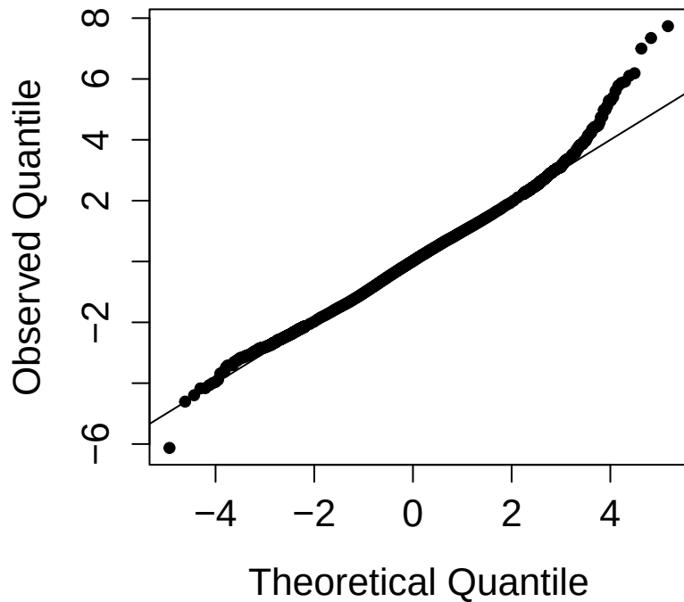
Fitted skew-t
