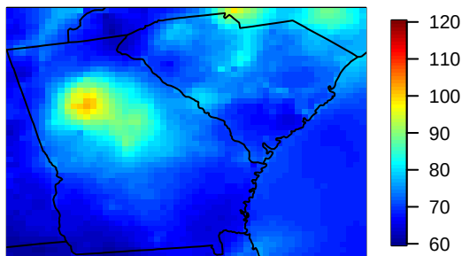
(b) Skew-t, K=1, T=0, No Time Series,
