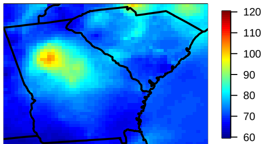
Skew-t, K=5, T=50, No Time Series
