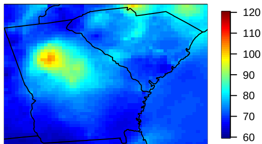
(c) Skew-t, K=5, T=50, No Time Series
