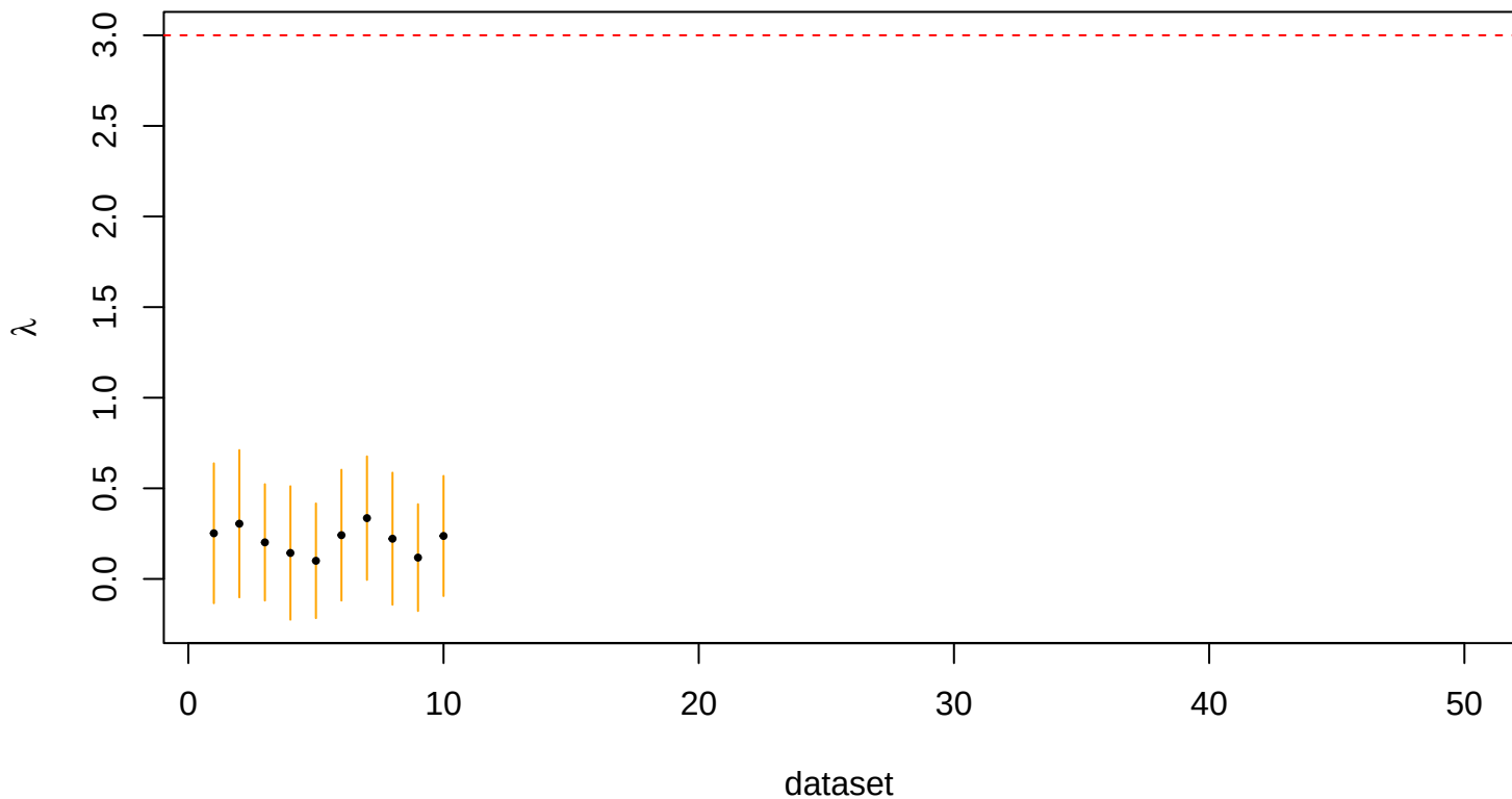
95% CI for lambda – method 2, mrts_k = 3
