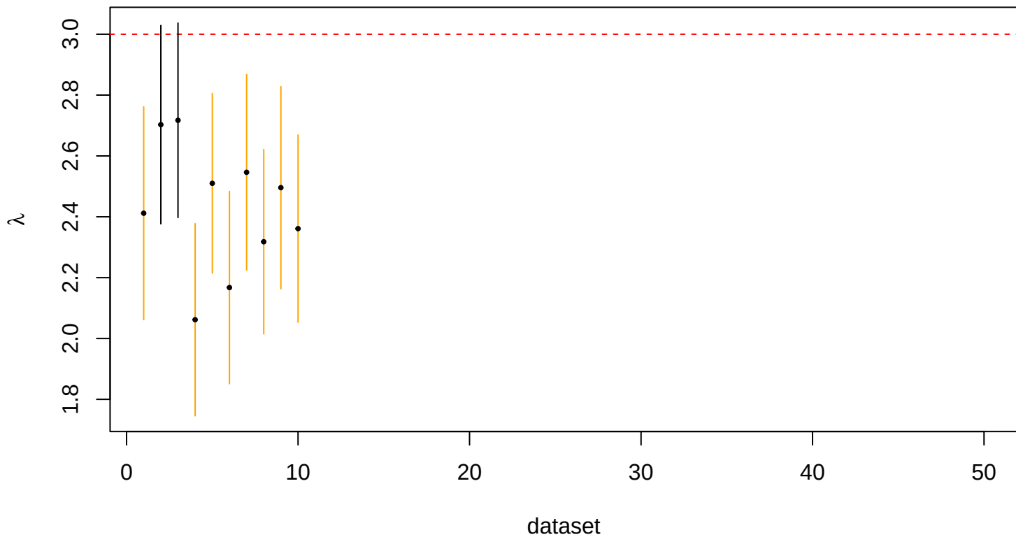
95% CI for lambda – method 4, mrts_k = 15
