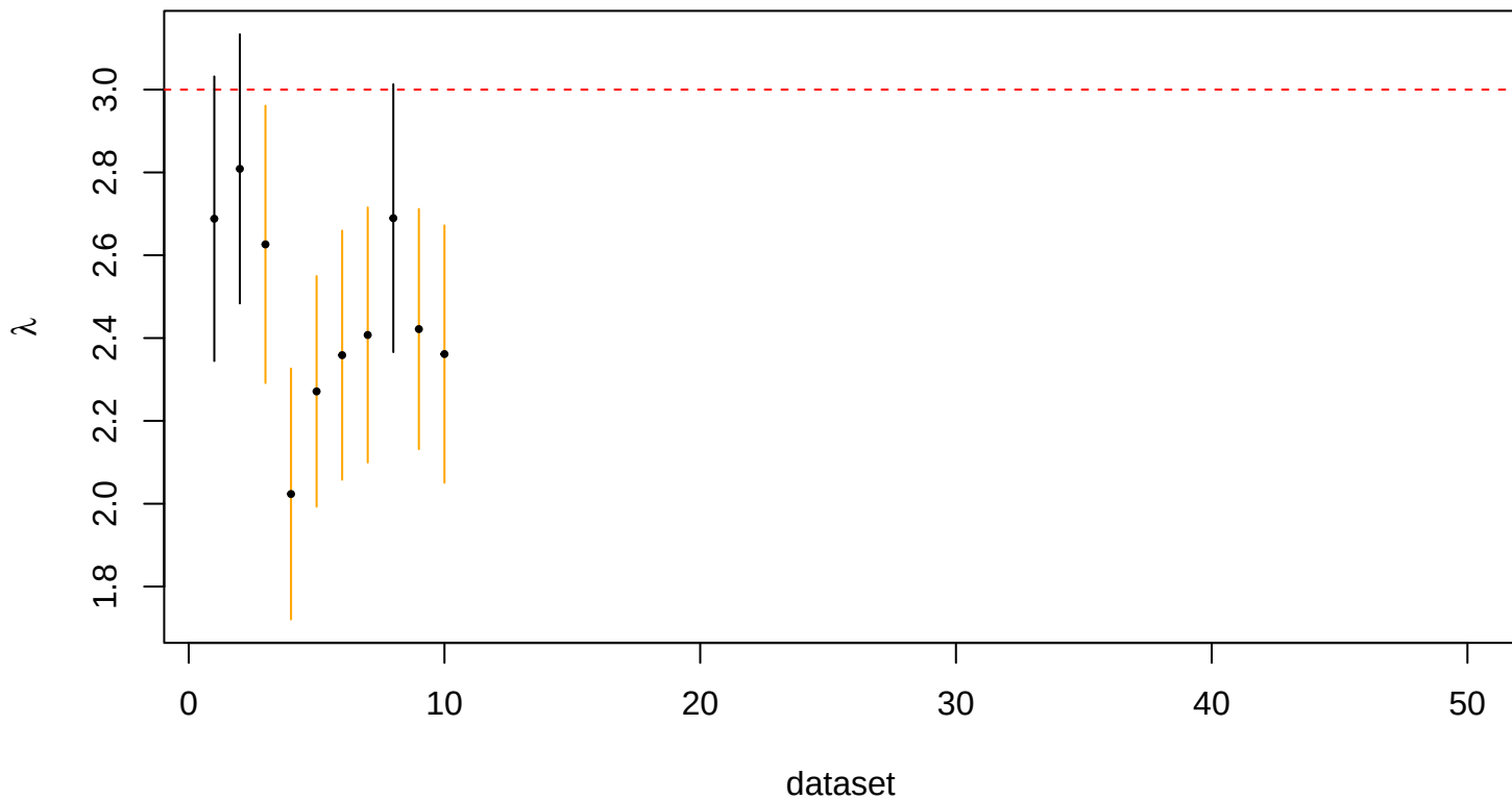
95% CI for lambda – method 4, mrts_k = 20
