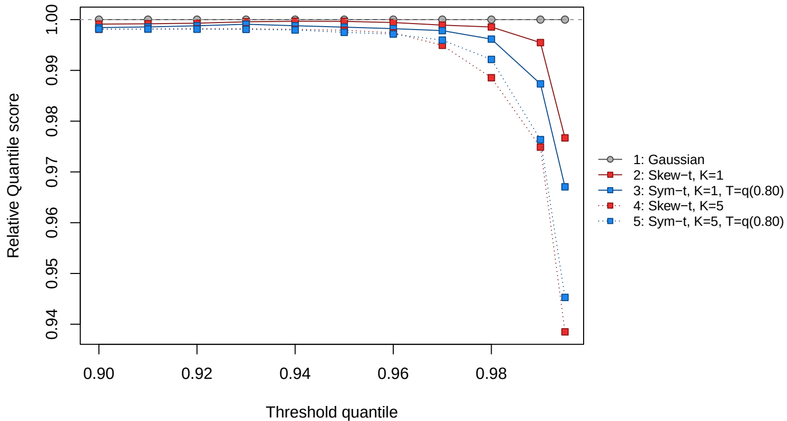
Skew- t ( K=5, \lambda=3 )
