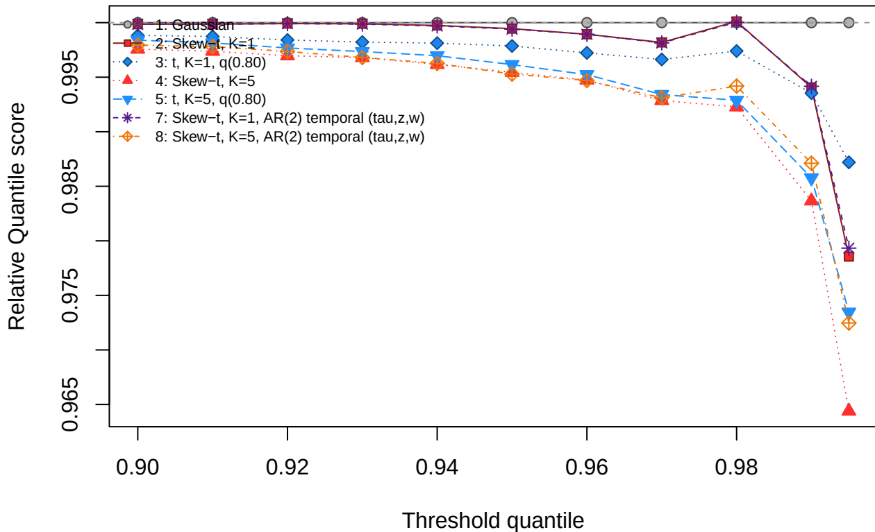
Skew- t ( K=1, \lambda=3 ), AR(2): \phi_1=0.12, \phi_2=-0.05
