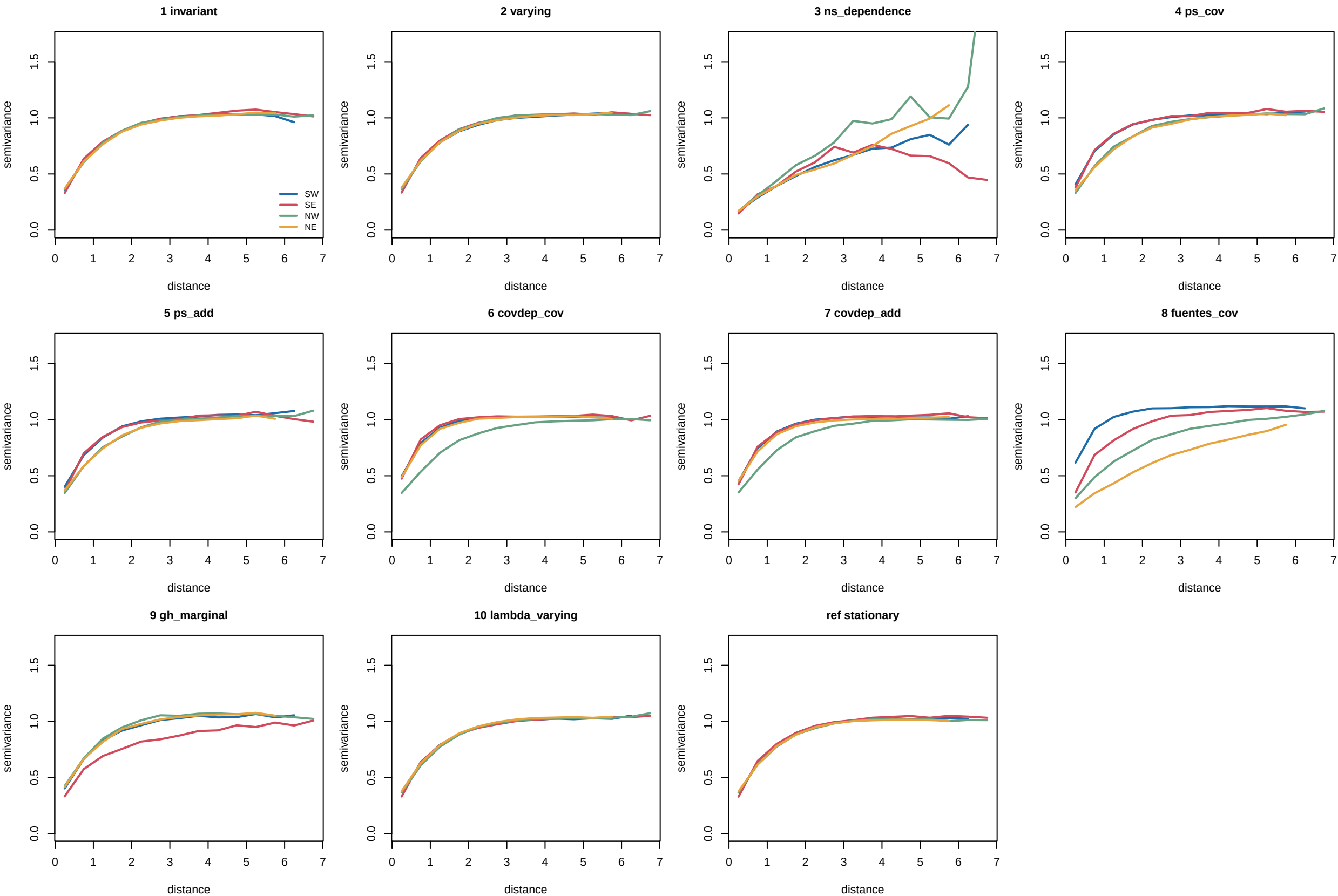
Variogram by quadrant -- curves SEPARATE \Leftrightarrow non-stationary dependence (compare the flat reference)
