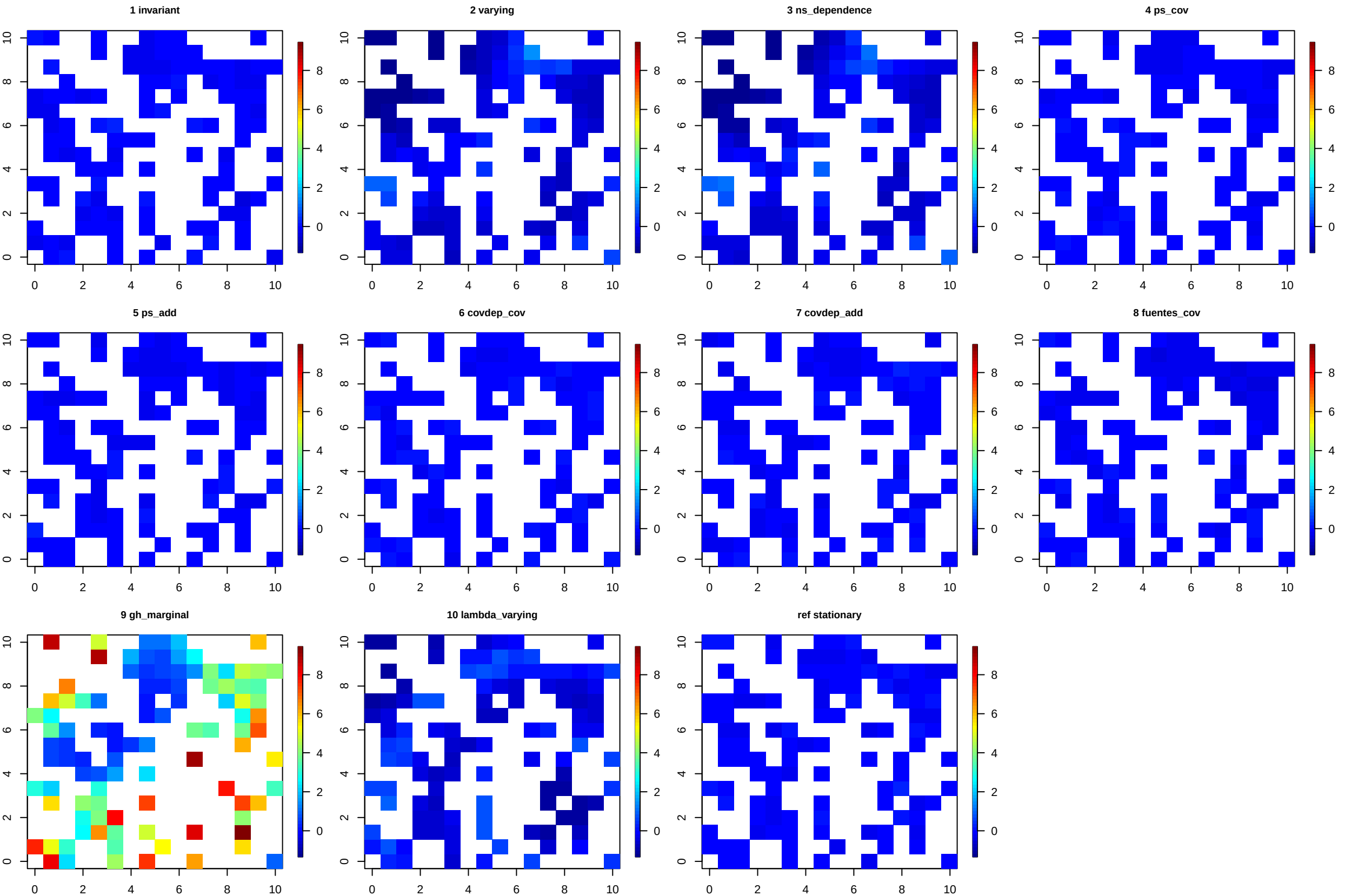
Pointwise excess kurtosis -- setting 9 should track h(s)
