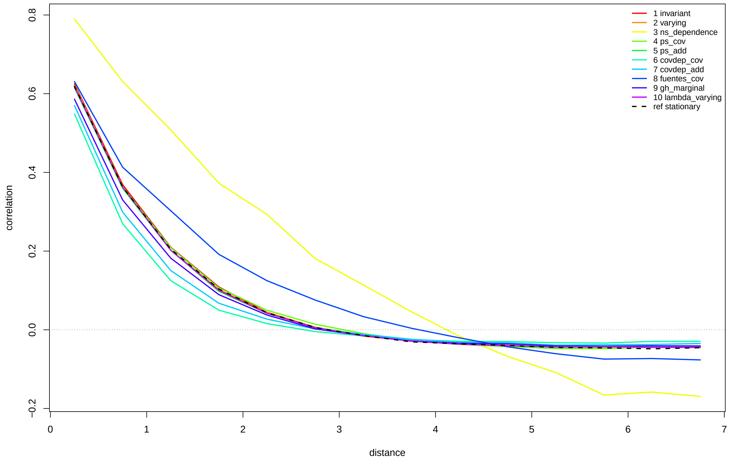
Pooled correlation vs distance setting 3's low-rank cosine basis goes NEGATIVE at long range -- a monotone Matern cannot
