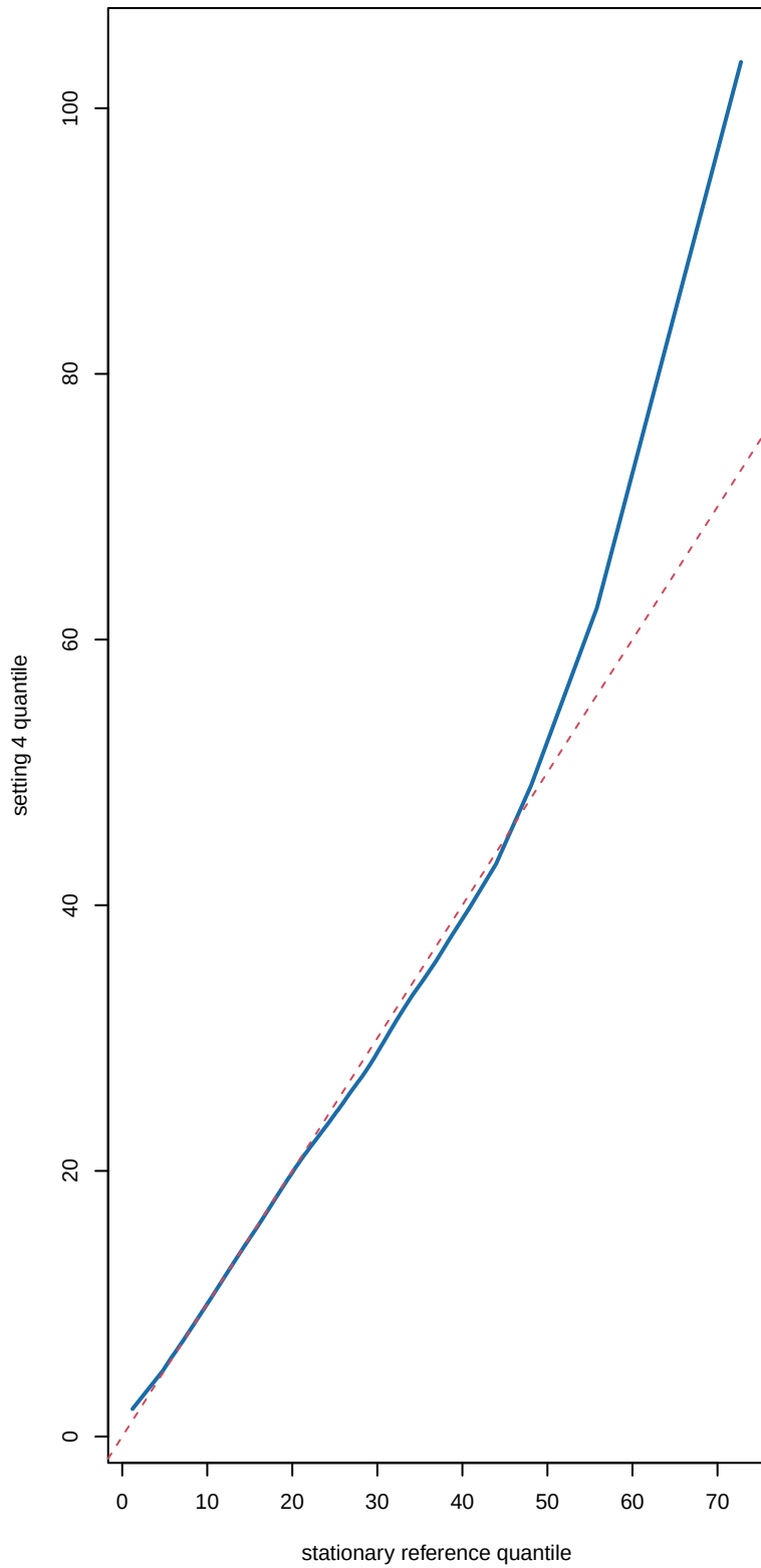
4 ps_cov
