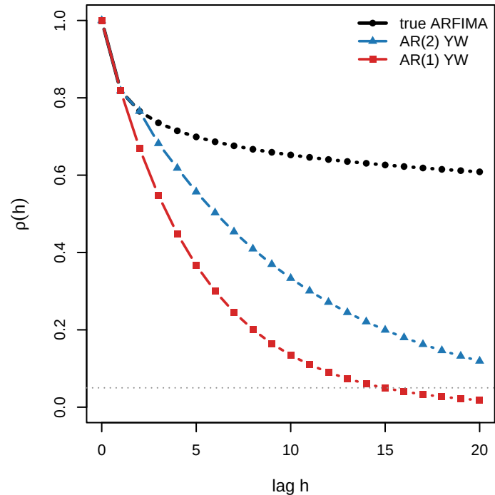
setting 19: ARFIMA d = 0.45 (H = 0.95)
