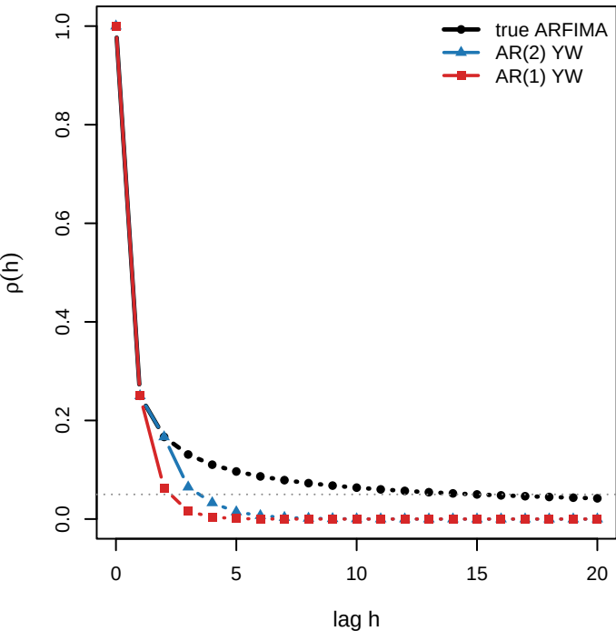
setting 17: ARFIMA d = 0.20 (H = 0.70)
