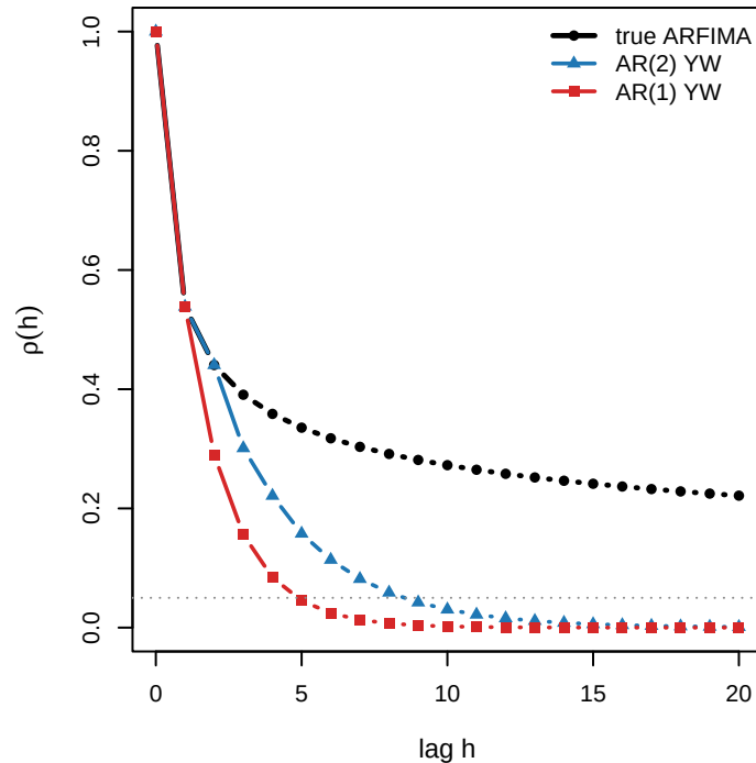
setting 18: ARFIMA d = 0.35 (H = 0.85)
