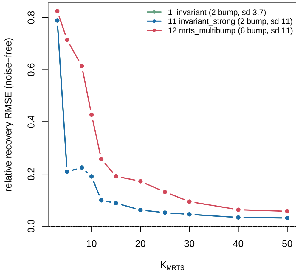
MRTS projection recovery vs K (the reason to want large K)
