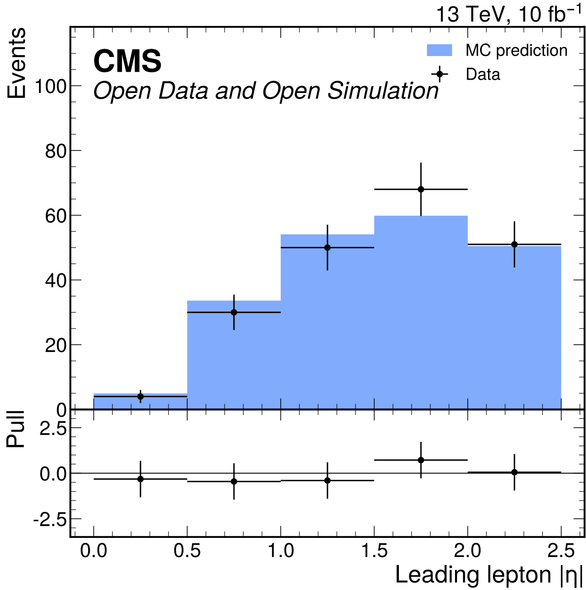
Figure 27: Leading lepton |\eta| input-validation distribution in the broad 70 less than or equal to m4l less than or equal to 170 GeV window. The D7 shape gate passes with \chi^2/\text{ndf} = 0.47344618565668173 and p = 0.7552866554534795 ; this comparison is used only to decide classifier-input eligibility, not to normalize fit templates.
