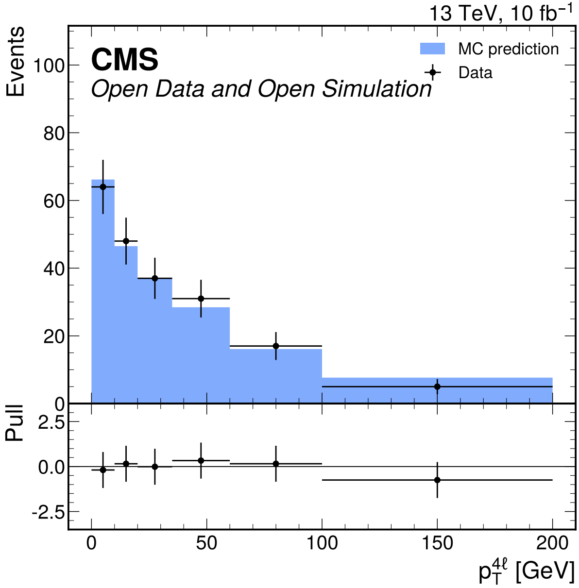
Figure 33: p_{T}^{4\ell} [GeV] input-validation distribution in the broad 70 less than or equal to m_{4\ell} less than or equal to 170 GeV window. The D7 shape gate fails with \chi^2/\text{ndf} = 0.33279924052380305 and p = 0.8934040385491403 ; this comparison is used only to decide classifier-input eligibility, not to normalize fit templates.
