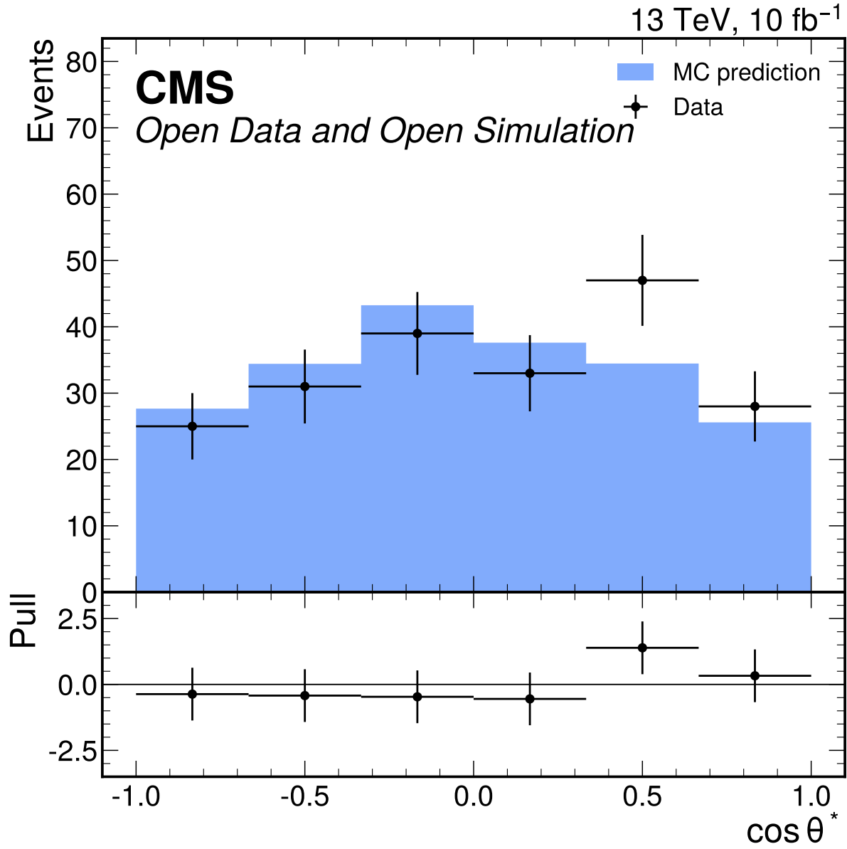
Figure 25: \cos\theta^* input-validation distribution in the broad 70 less than or equal to m_{4l} less than or equal to 170 GeV window. The D7 shape gate fails with \chi^2/\text{ndf} = 1.007137007365913 and p = 0.4115406899048306 ; this comparison is used only to decide classifier-input eligibility, not to normalize fit templates.
