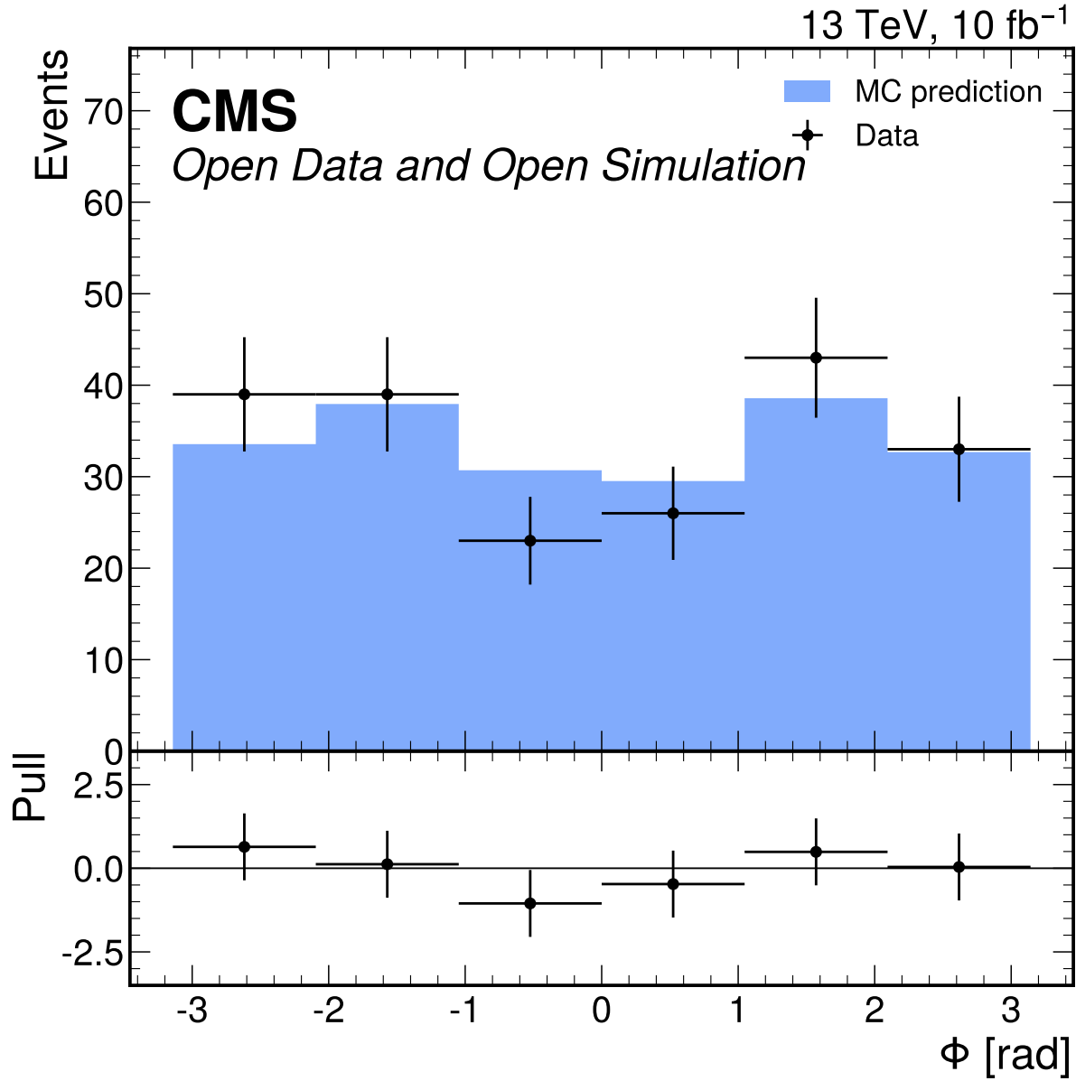
Figure 31: \Phi [rad] input-validation distribution in the broad 70 less than or equal to m_{4l} less than or equal to 170 GeV window. The D7 shape gate fails with \chi^2/\text{ndf} = 0.780243891250844 and p = 0.5637239206342102 ; this comparison is used only to decide classifier-input eligibility, not to normalize fit templates.
