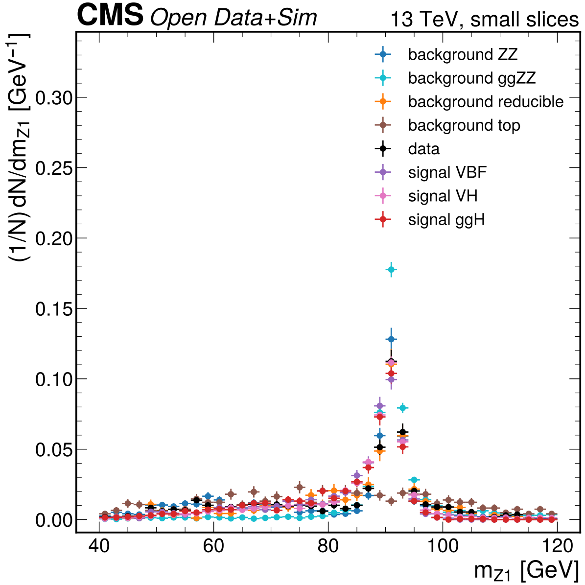
Figure 18: m_{Z1} [GeV] small-slice shape comparison. The distributions use at most 1000 entries per primary ROOT file and are area-normalized only for Phase 1 shape reconnaissance, not for yield validation. Large differences here flag candidate variables for Phase 2/3 data-MC quality checks rather than final selection conclusions.
