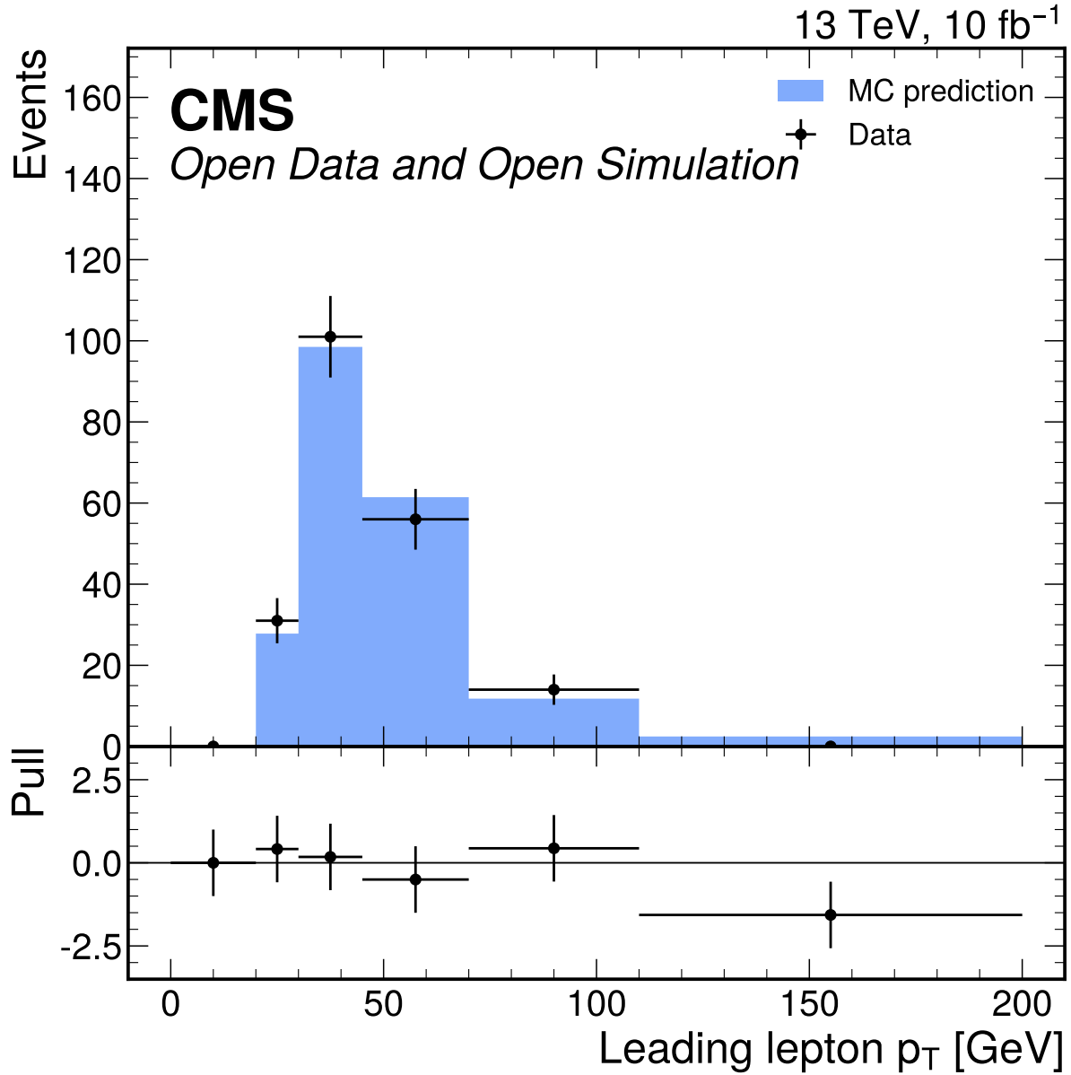
Figure 28: Leading lepton p_T [GeV] input-validation distribution in the broad 70 less than or equal to m_{4l} less than or equal to 170 GeV window. The D7 shape gate fails with \chi^2/\text{ndf} = 4.056365380026655 and p = 0.0027310794648283346 ; this comparison is used only to decide classifier-input eligibility, not to normalize fit templates.
