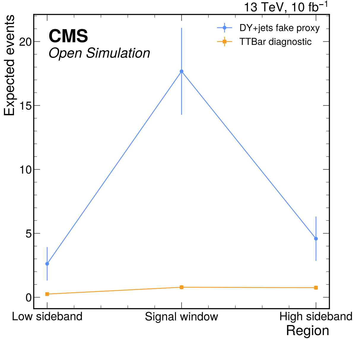
Figure 42: DY+jets fake proxy and TTBar diagnostic reducible-background checks across the predeclared sideband and signal regions. TTBar diagnostic / DY+jets fake-proxy ratios are {'high_sideband_140_170': 0.16348247967166454, 'low_sideband_70_105': 0.09536477980847097, 'signal_window_105_140': 0.04440264879971137}, so TTBar is not promoted to the nominal fake model by the Phase 2 thresholds.
