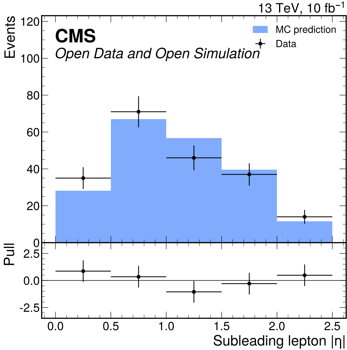
Figure 34: Subleading lepton |\eta| input-validation distribution in the broad 70 less than or equal to m4l less than or equal to 170 GeV window. The D7 shape gate fails with \chi^2/\text{ndf} = 1.0759966157041323 and p = 0.36642617632066843 ; this comparison is used only to decide classifier-input eligibility, not to normalize fit templates.
