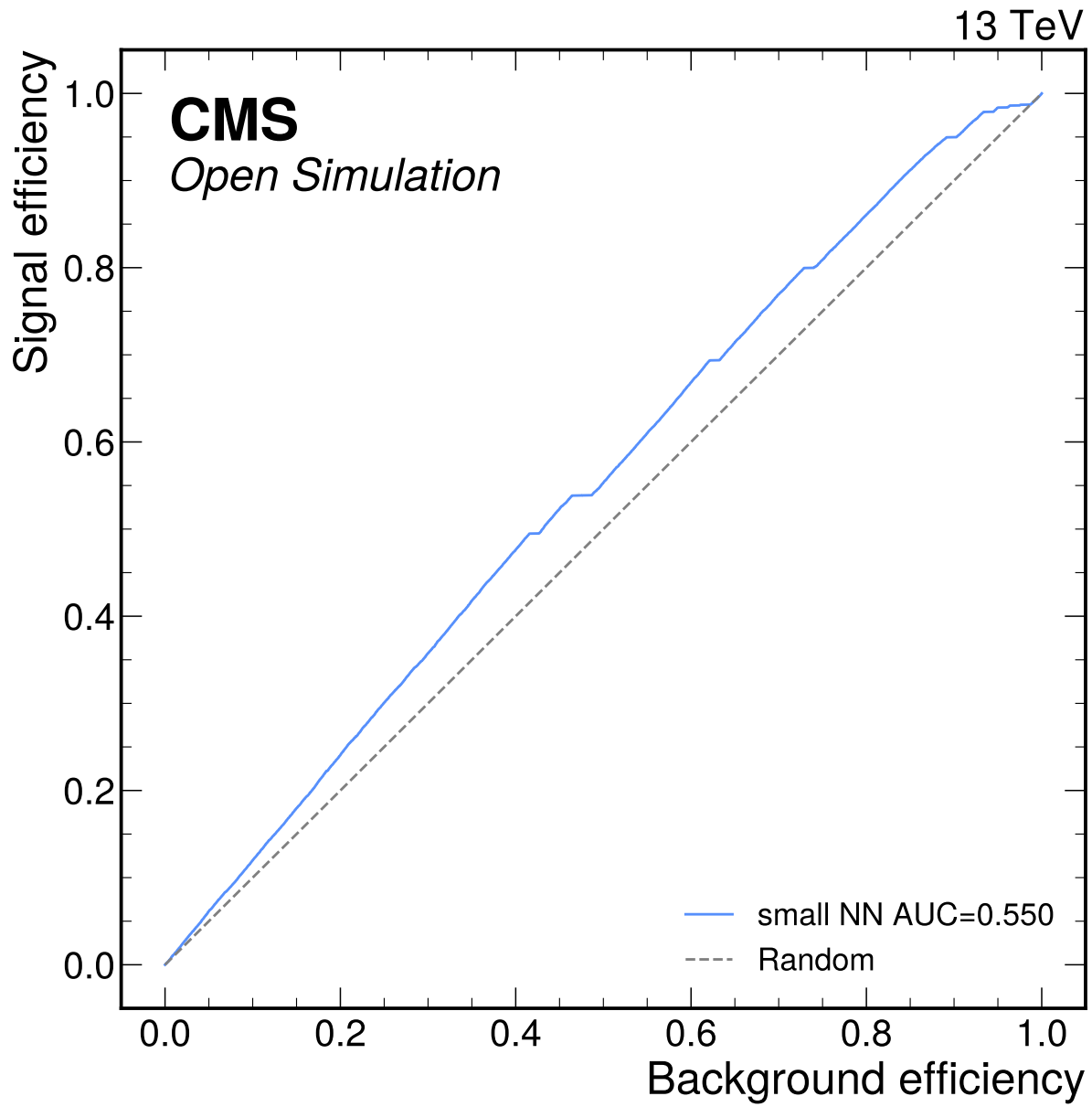
Figure 58: Small NN classifier ROC curve for the S2 attempt. The neural-network route is preserved as rejected-approach evidence and is not used to define the active signal-strength categories.
