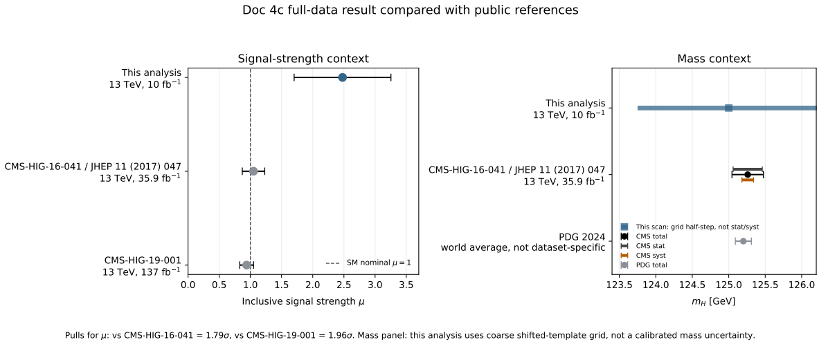
Figure 24: Full-data signal-strength and mass-diagnostic comparison with public CMS and PDG references. The labels state the center-of-mass energy and luminosity for dataset-specific entries; the PDG entry is labeled as a world average rather than a dataset. The signal-strength pulls are 1.79 standard deviations relative to CMS-HIG-16-041 and 1.96 standard deviations relative to CMS-HIG-19-001. In the mass panel, CMS-HIG-16-041 shows separate statistical and systematic uncertainty bars plus the total uncertainty, while this analysis is shown with a coarse grid half-step only to emphasize that the shifted-template scan is diagnostic and not a calibrated mass measurement.
