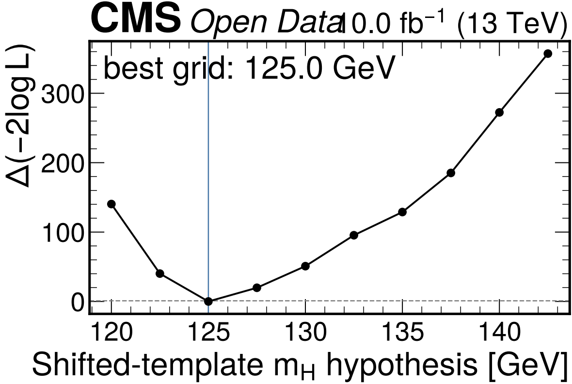
Figure 23: Observed shifted-template detector-level mass scan with \mu profiled at each mass hypothesis. The best grid point is 125.0 GeV, but the scan is not an official CMS-quality mass measurement because independent mass-hypothesis MC and official calibration/morphing inputs are unavailable.
