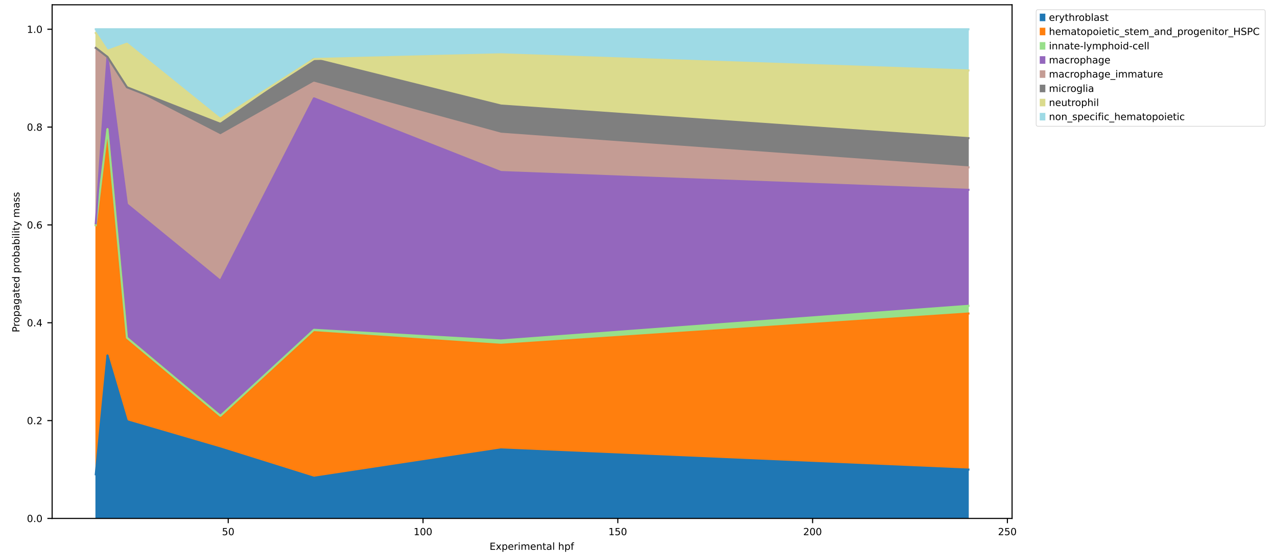
Combined-model push-forward from earliest observed HSPCs
