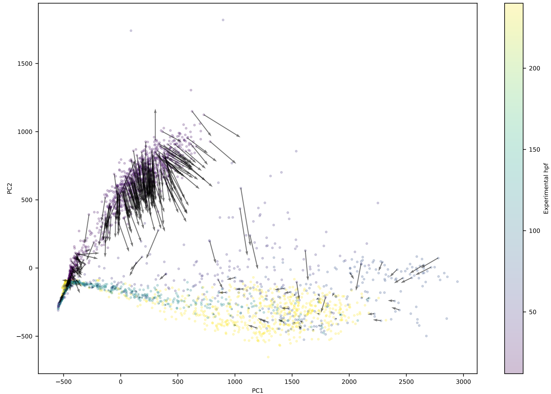
moscot x GraphVelo real-time finite-difference velocities
