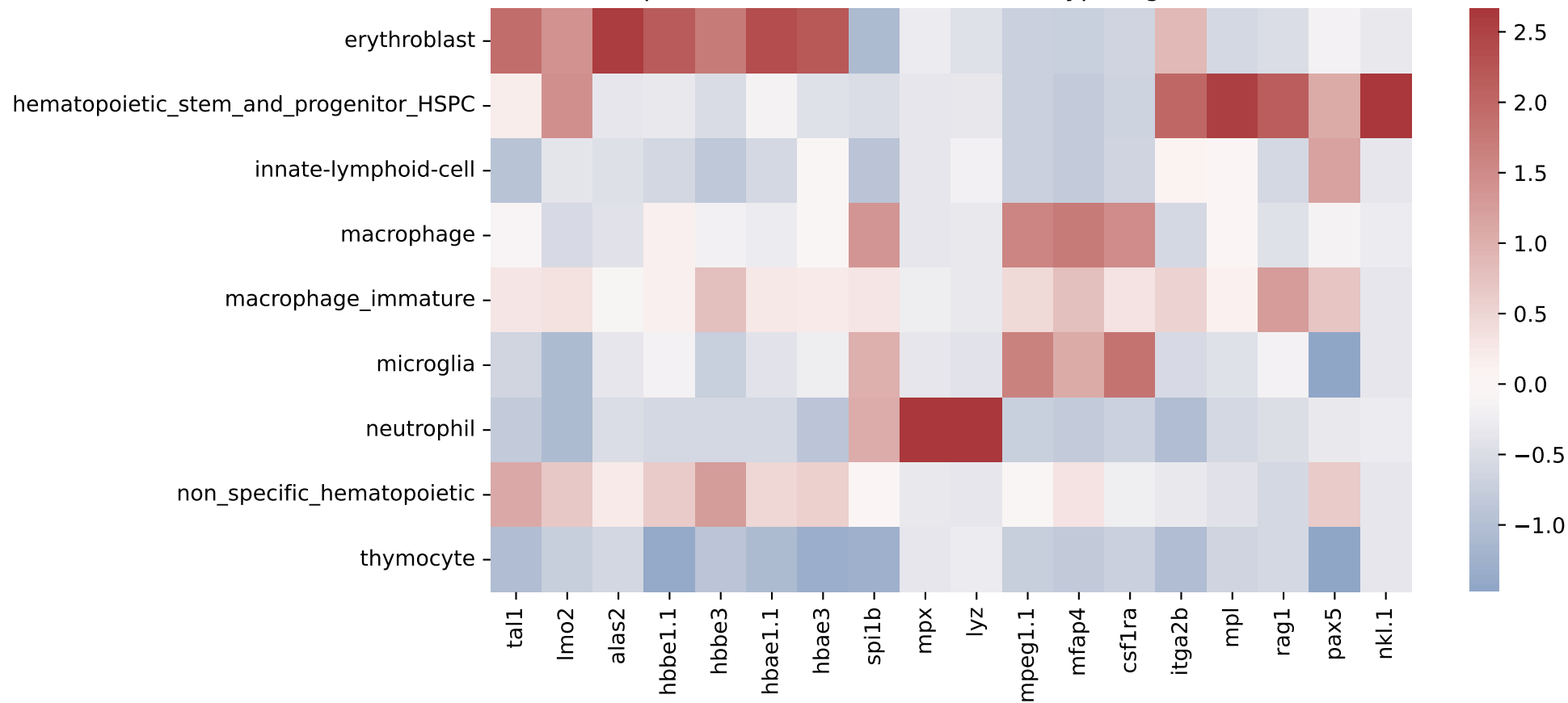
Marker expression across official fine cell types (gene-wise z-score)
