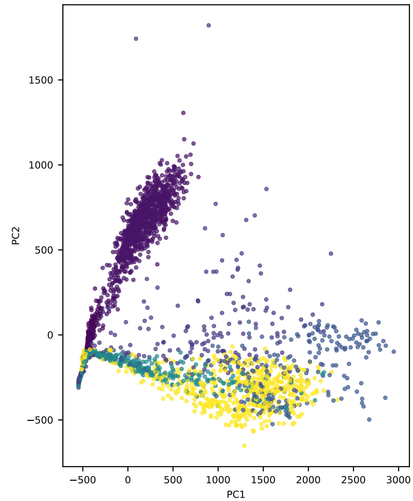
PCA state space by experimental hpf
