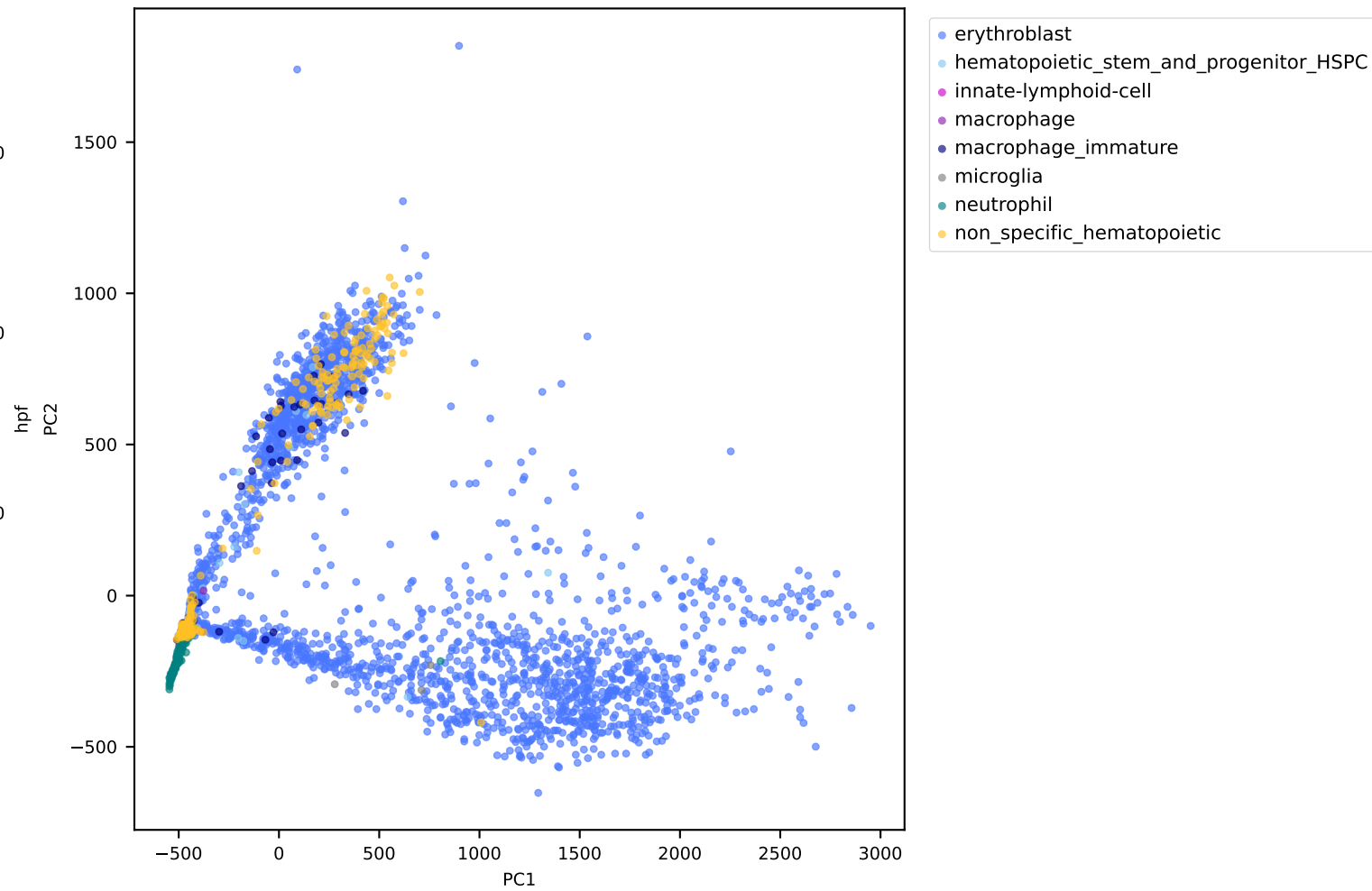
PCA state space by official fine annotation
