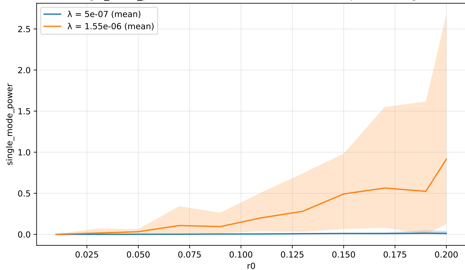
single_mode_power vs r0 — mean with min-max band per wavelength
