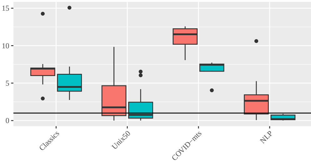
Speedup vs. bash
