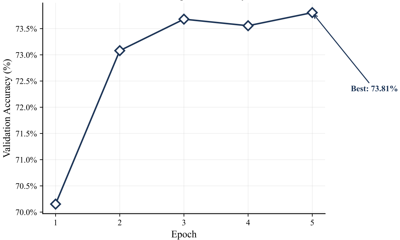
Validation Argmax Accuracy
