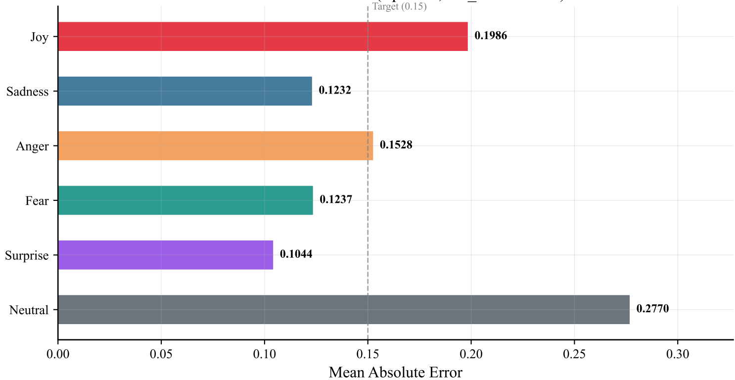
Per-Dimension MAE (Epoch 5, val_loss=0.7272)
