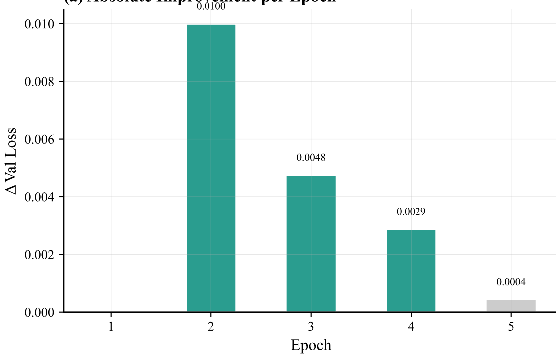
(a) Absolute Improvement per Epoch
