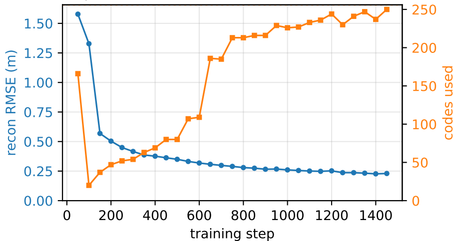
etrain — depth recon vs codebook utilisation (EMA + dead-c
