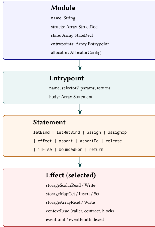
Figure 2: Portable IR module structure. A Module contains state declarations and typed entrypoints. Each entrypoint body is a sequence of statements, which may produce typed effects that carry capability identifiers.
