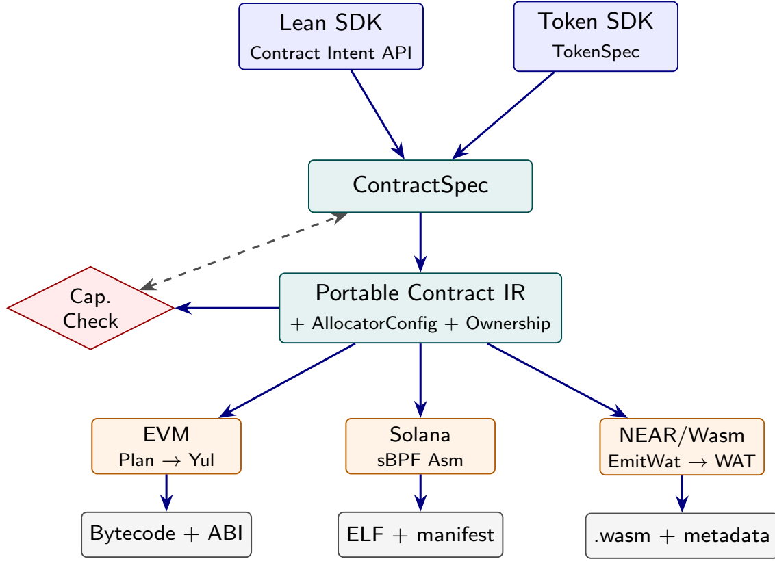
Figure 1: ProofForge compilation pipeline. Lean source lowers through ContractSpec to a portable IR, which is routed via capability checks to target-specific backends. Unsupported capabilities are rejected before artifact generation.
