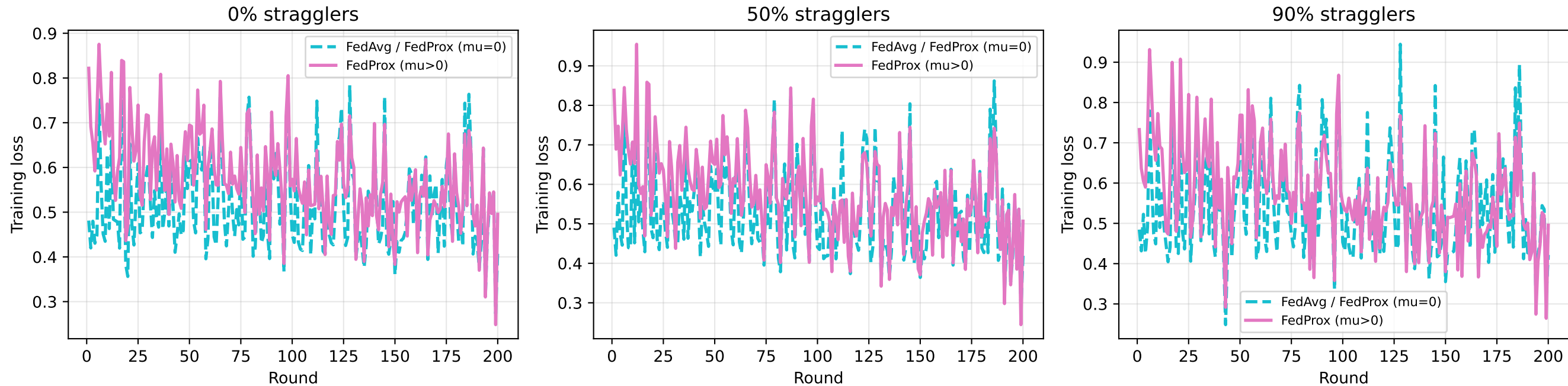
Figure 1: FedProx vs FedAvg under systems heterogeneity (stragglers)
