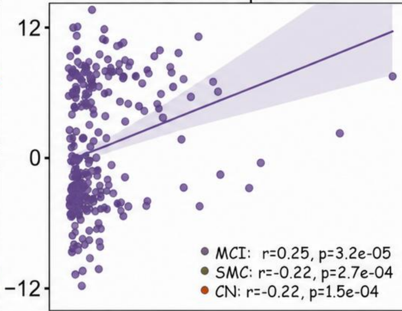
PTau217 / a \beta 42 ratio
