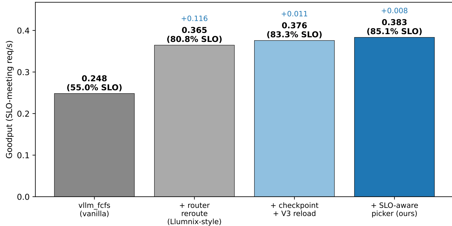
4-baseline ablation @ dual arxivsumm QPS=0.5 (mean of seed 0,1)
