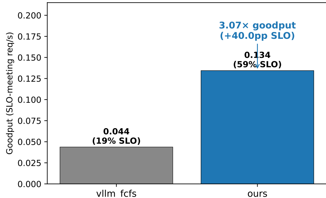
Single GPU, arxivsumm @ QPS=0.25 (mean of seed 0,1)
