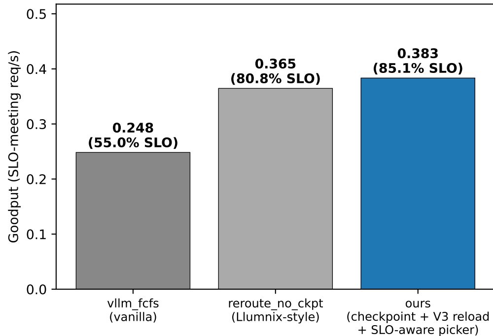
Dual GPU, arxivsumm @ QPS=0.5 (mean of seed 0,1)
