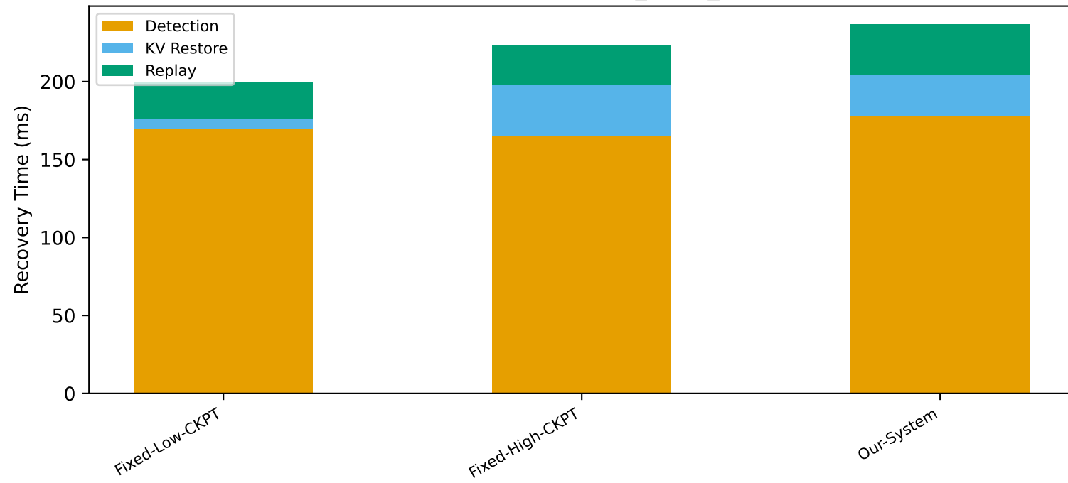
Recovery Breakdown — W1_Short_Interactive
