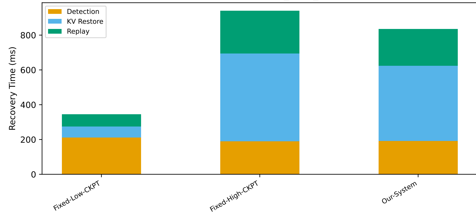
Recovery Breakdown — W2_Long_Generation
