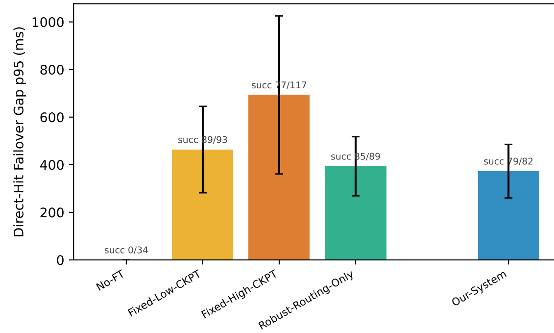
Direct-Hit Failover Gap — W2_Long_Generation
