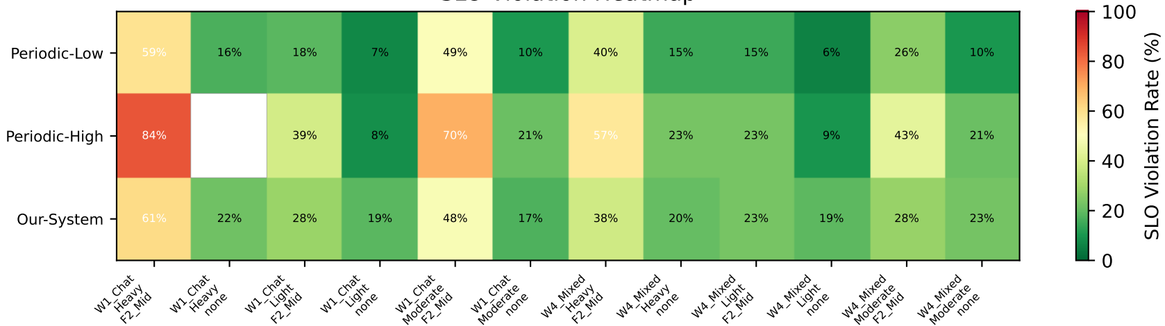
SLO Violation Heatmap
