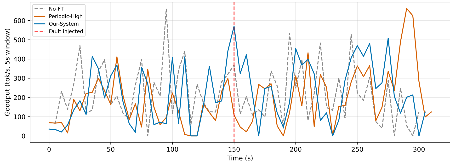
Goodput Timeline Around Fault
