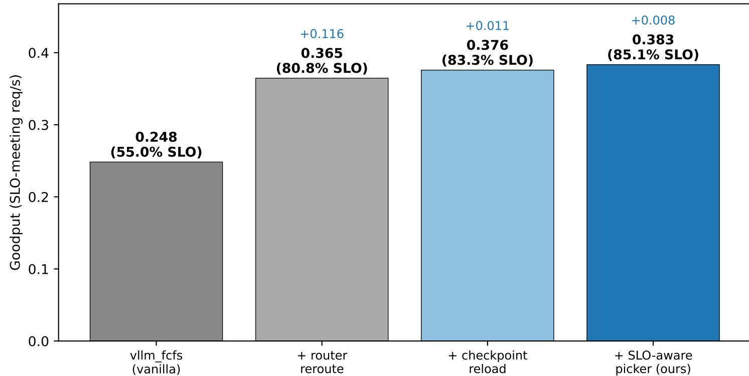
4-baseline ablation @ two-engine arxivsumm QPS=0.5 (mean of seed 0,1)
