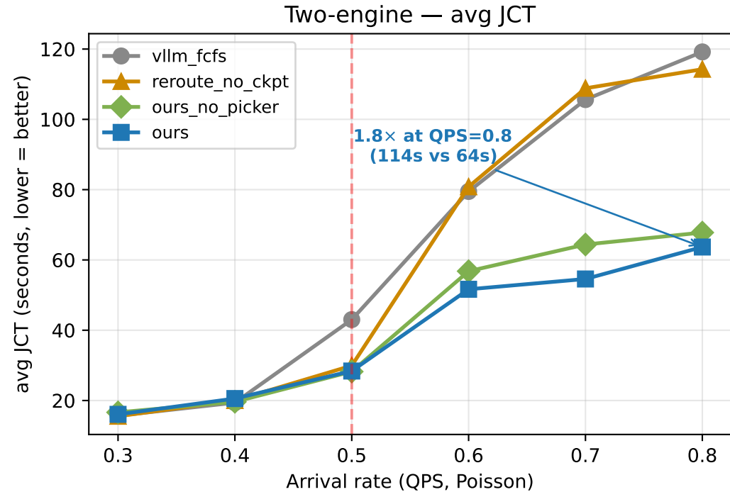
Two-engine arxivsumm — Job Completion Time (mean of seed 0,1)
