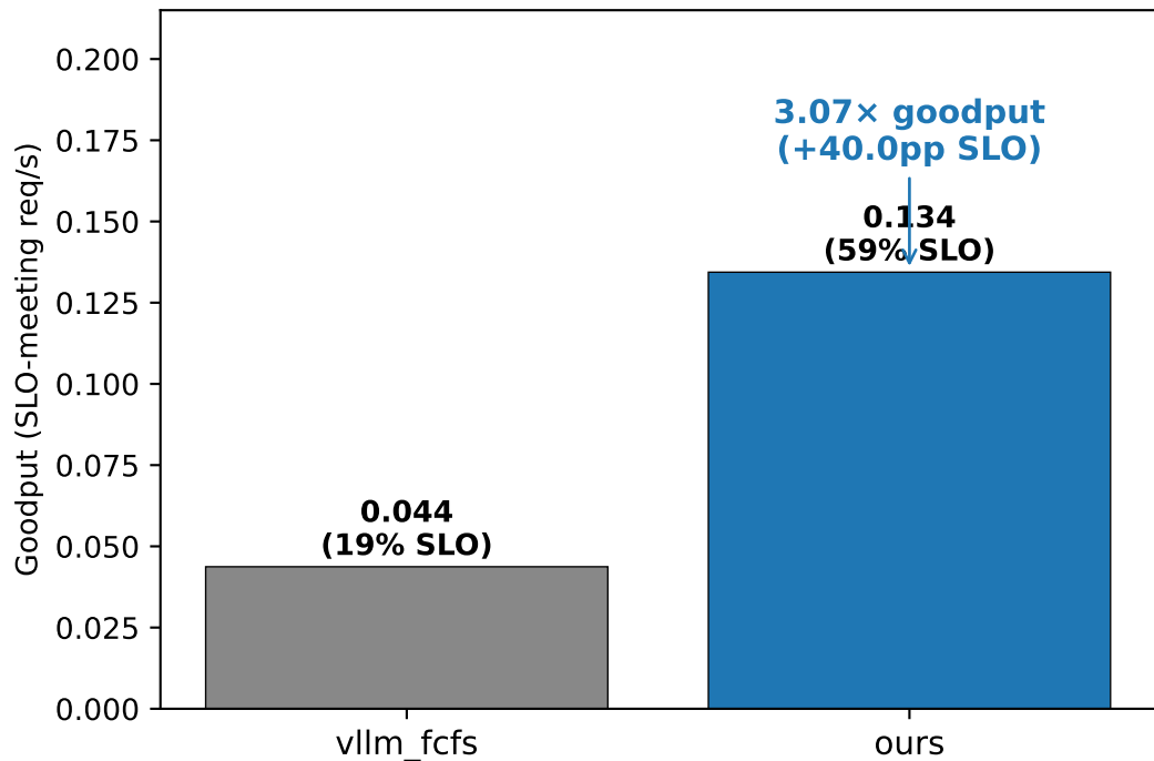
Single-engine, arxivsumm @ QPS=0.25 (mean of seed 0,1)
