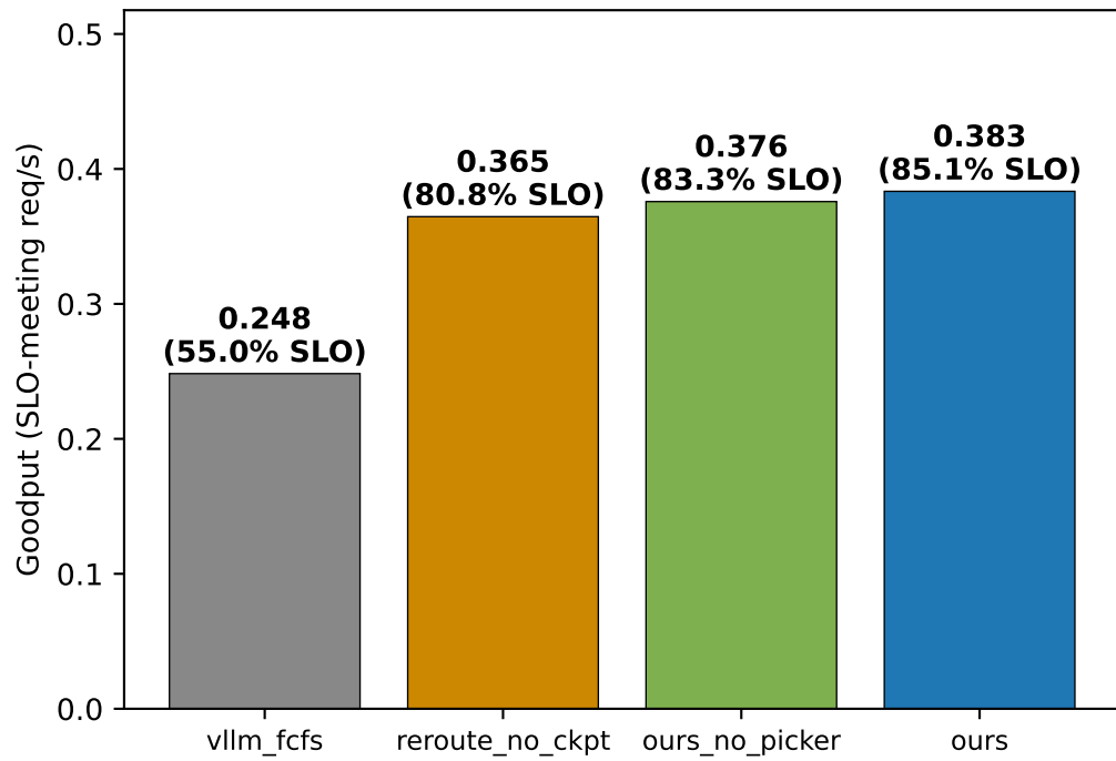
Two-engine, arxivsumm @ QPS=0.5 (mean of seed 0,1)
