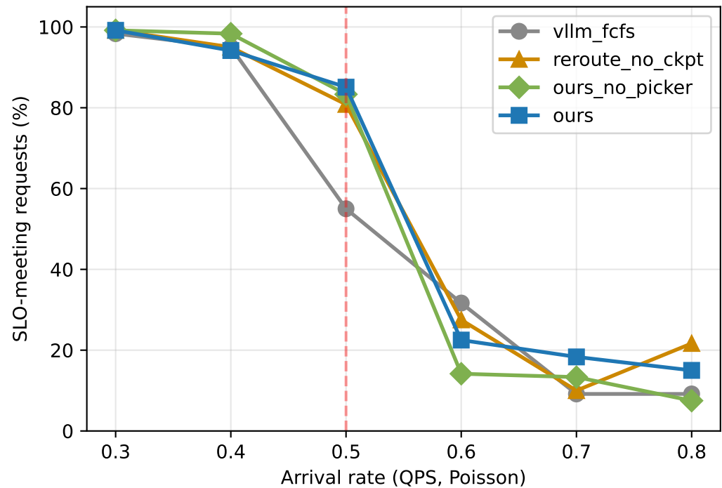
SLO attainment vs load (mean of seed 0,1)
