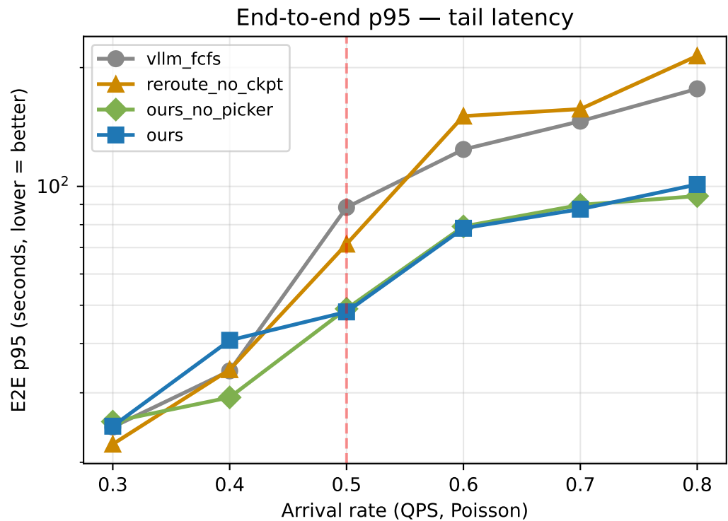
Two-engine arxivsumm tail latency (mean of seed 0,1)
