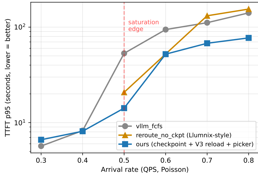
TTFT p95 — tail latency
