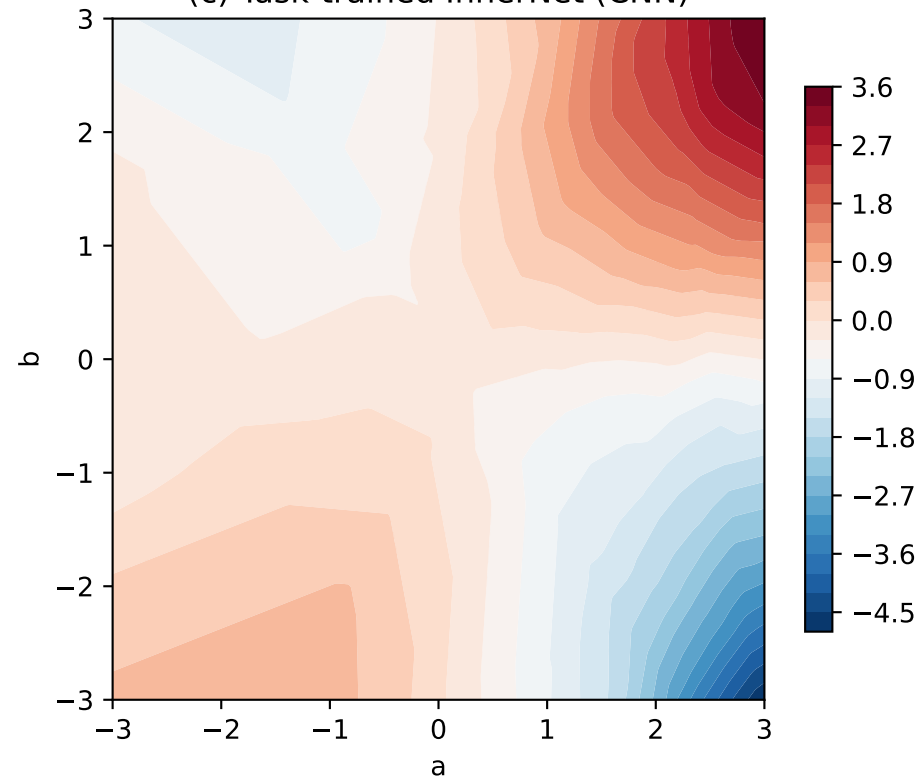
(c) Task-trained InnerNet (CNN)
