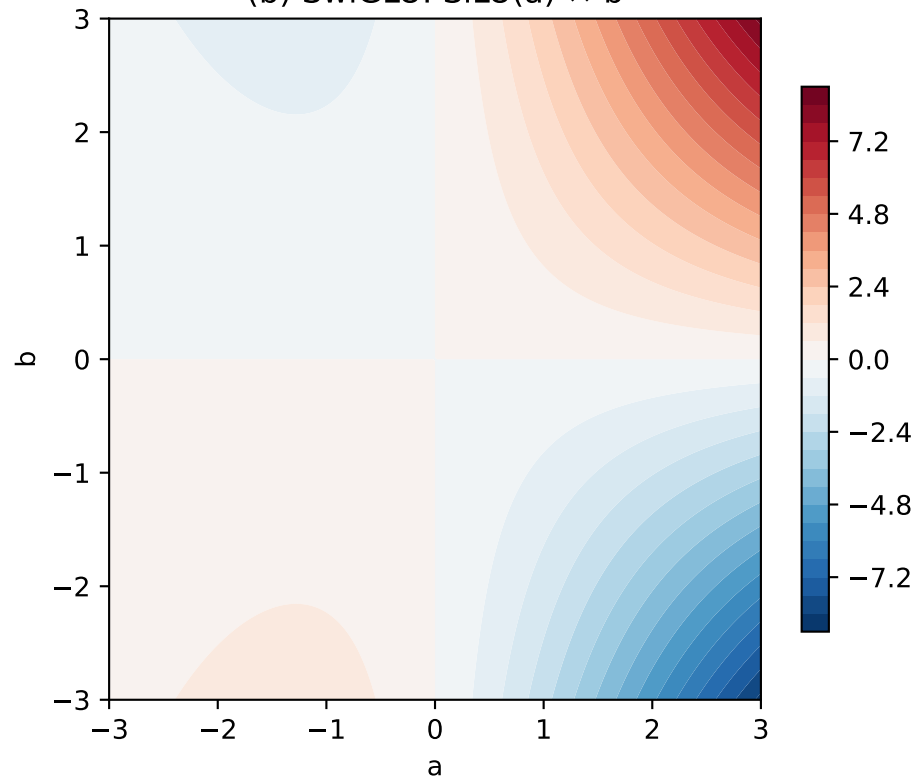
(b) SwiGLU: \text{SiLU}(a) \times b
