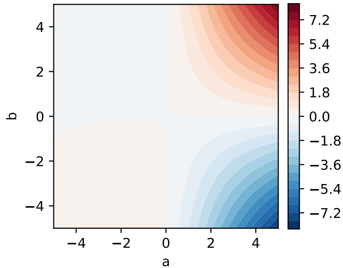
Scaled SwiGLU fit ( R^2=0.977 )
