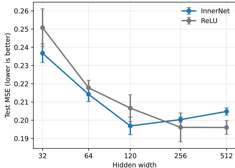
Housing regression (3 seeds)
