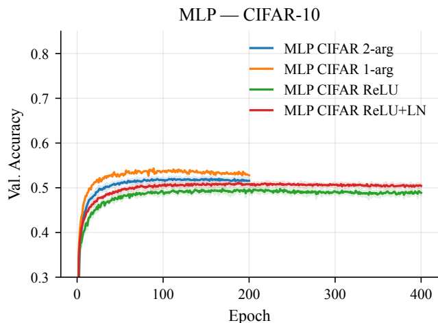
Training curves (mean \pm sample SD across seeds)
