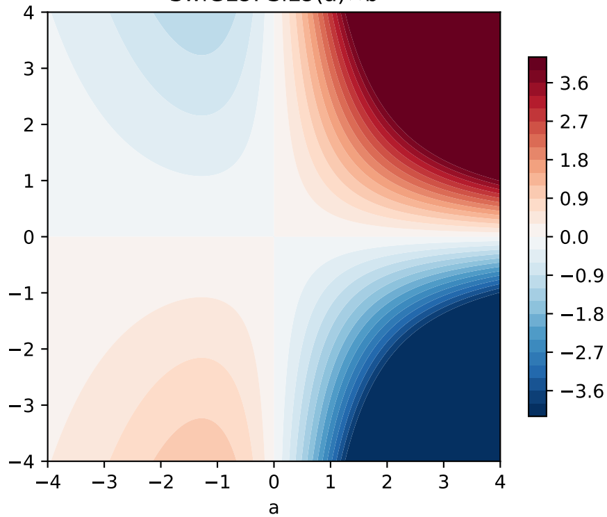
SwiGLU: SiLU(a)×b
