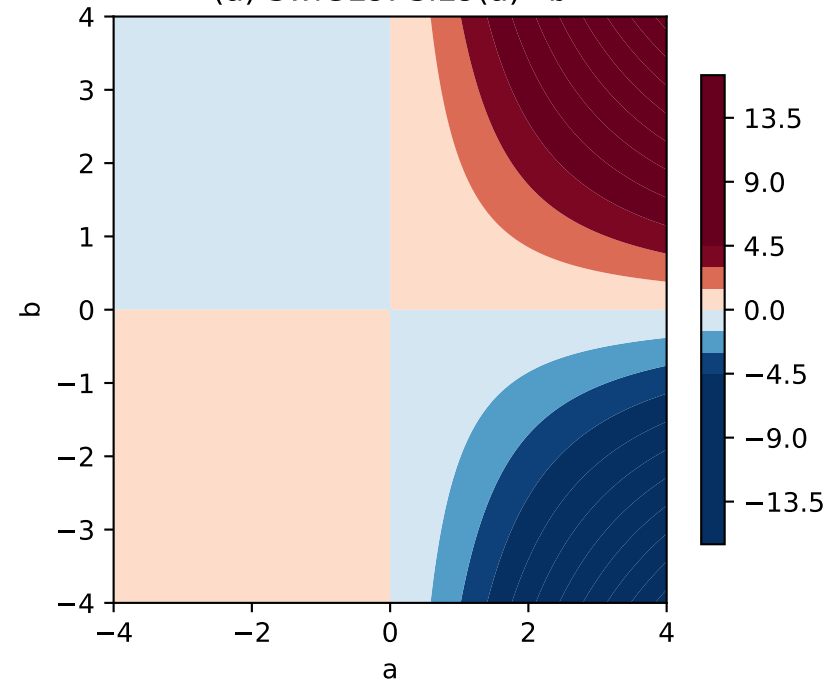
(a) SwiGLU: \text{SiLU}(a) \times b
