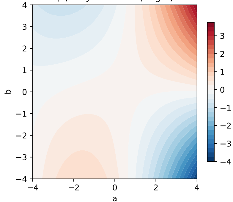
(c) Polynomial fit (deg 4)
