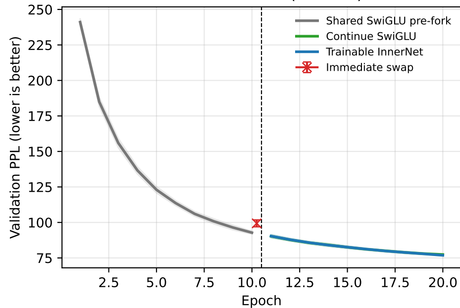
Warm-start fork (5 seeds)
