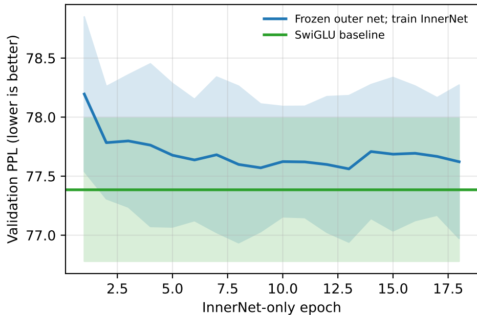
Frozen-capacity test (first 18 epochs)
