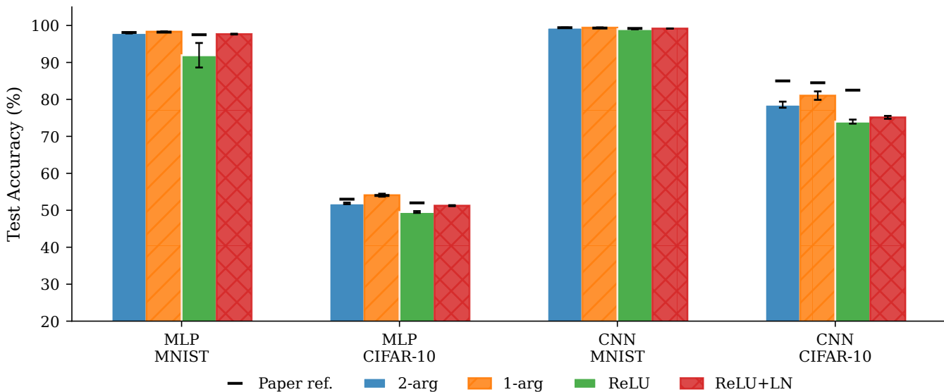
Classification Accuracy (Figure 4d)
