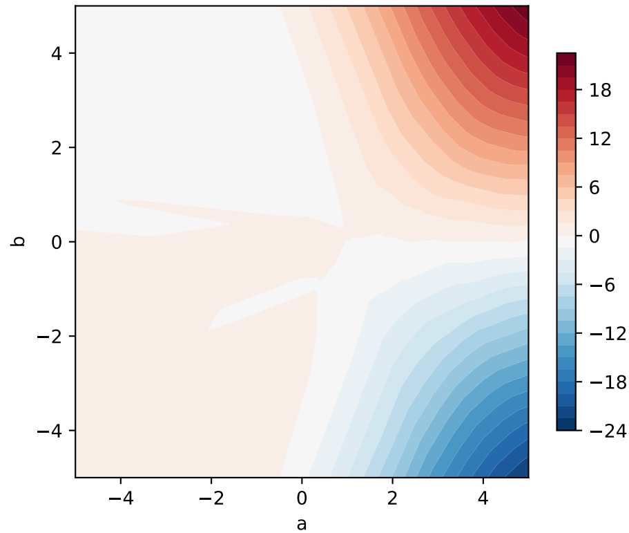
(b) InnerNet fitted to SwiGLU
