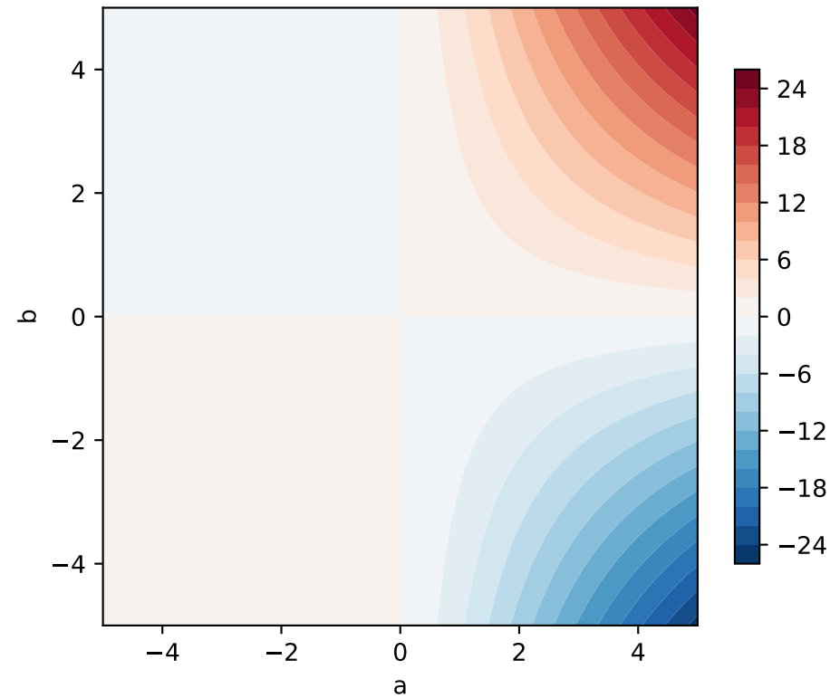
(a) SwiGLU: \text{SiLU}(a) \times b
