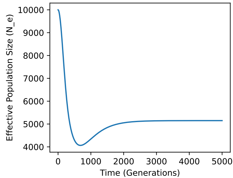
N=5000, U=0.0004, s=0.002
