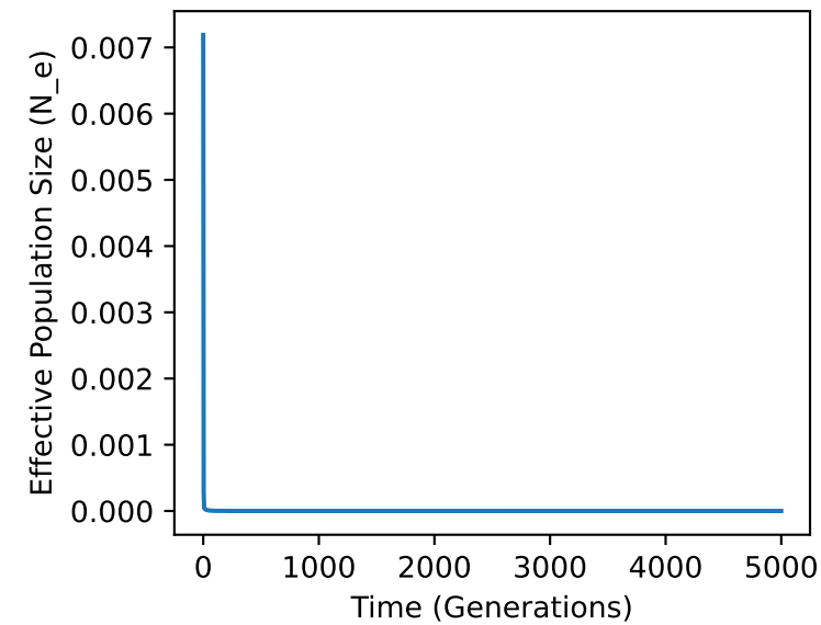
N=5000, U=0.006, s=0.01
