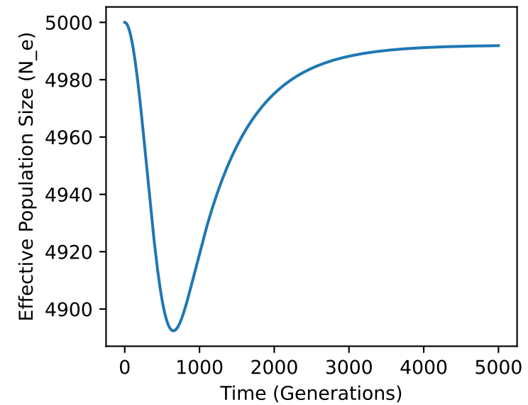
N=5000, U=0.006, s=0.0004
