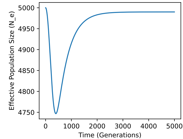
N=5000, U=0.006, s=0.002
