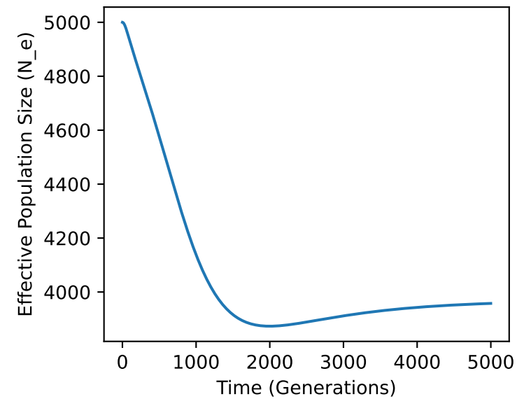
N=5000, U=0.01, s=0.002
