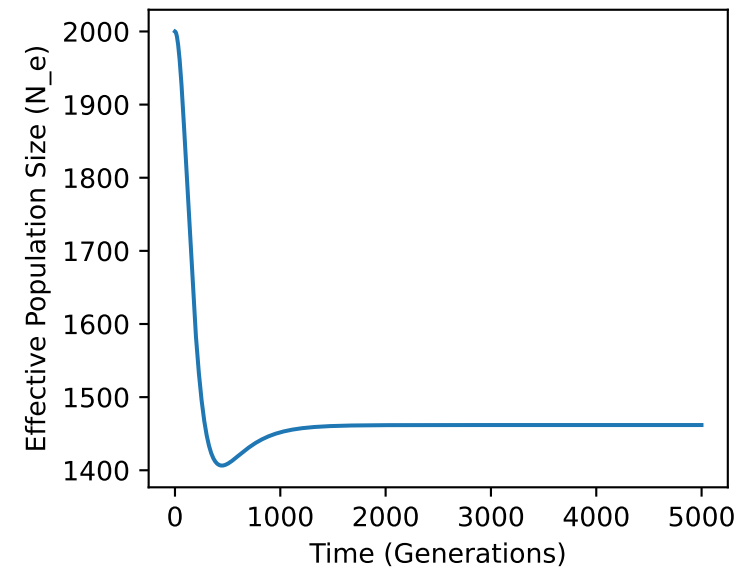
N=5000, U=0.006, s=0.0001
