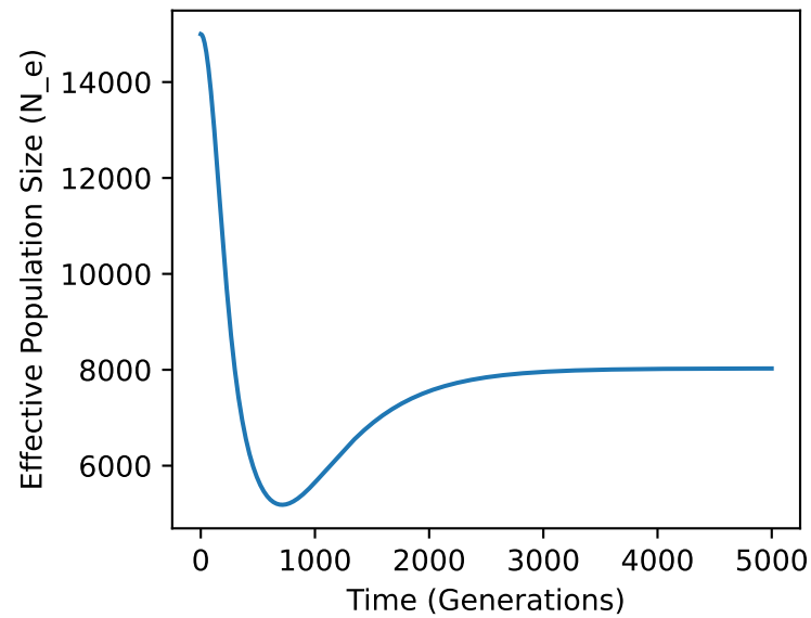
N=5000, U=0.006, s=0.0
